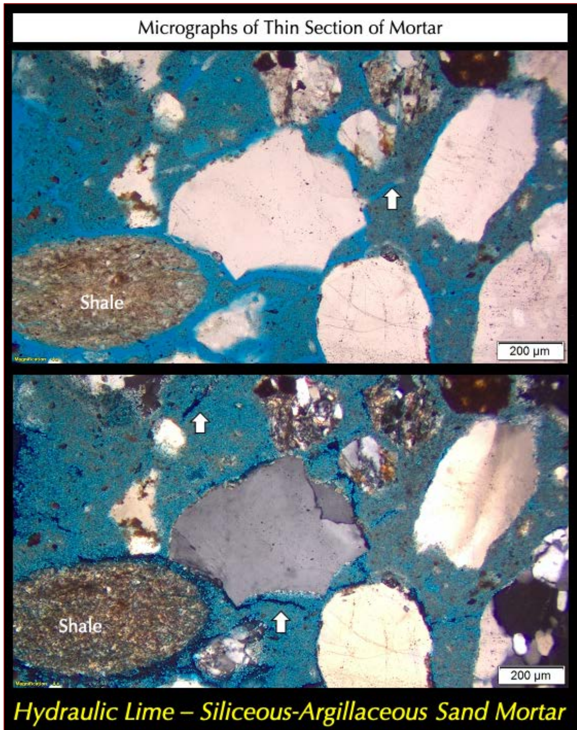
Figure 18: Micrographs of thin section of mortar showing: (a) non-air-entrained nature of mortar; (b) subangular to subrounded, mostly equidimensional siliceous-argillaceous sand particles that are nominal 2 mm in size, well-graded, well-distributed, consisting of major amount of variably strained quartz and subordinate amounts of quartzite, feldspar, quartz siltstone, and other siliceous particles; and a subordinate amount of shale, ferruginous and argillaceous siltstone particles, and (c) carbonated hydraulic lime paste. Top photo shows the plane polarized view to highlight sand particles, carbonation shrinkage microcracks (a few are marked with arrows) and voids, whereas bottom photo shows corresponding cross polarized light image to show the sand types and carbonated paste.
