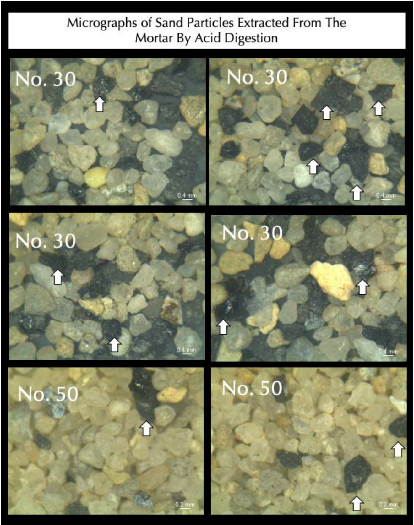
Figure 5: Micrographs of extracted sand particles from the mortar retained on various sieves. Arrows show some dark particles in sand.
