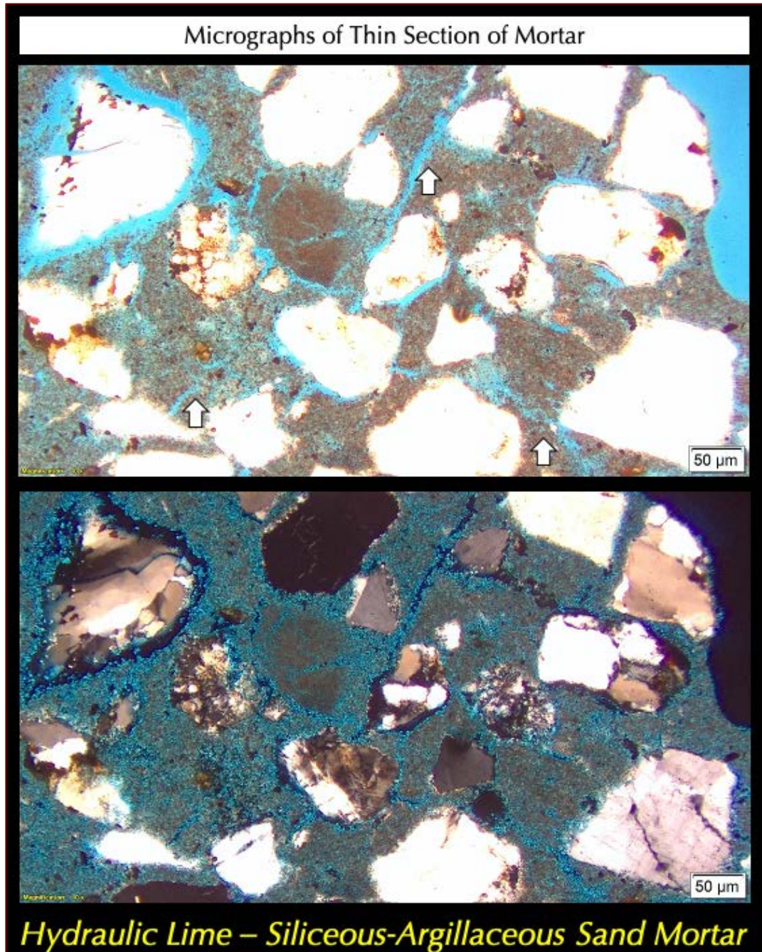
Figure 12: Micrographs of thin section of mortar showing: (a) non-air-entrained nature of mortar; (b) subangular to subrounded, mostly equidimensional siliceous-argillaceous sand particles that are nominal 2 mm in size, well-graded, well-distributed, consisting of major amount of variably strained quartz, and subordinate amounts of quartzite, feldspar, quartz siltstone, and other siliceous particles; and a subordinate amount of shale, ferruginous and argillaceous siltstone particles, and (c) carbonated hydraulic lime paste. Top photo shows the plane polarized view to highlight sand particles, carbonation shrinkage microcracks (a few are marked with arrows) and voids, whereas bottom photo shows corresponding cross polarized light image to show the sand types and carbonated paste.
