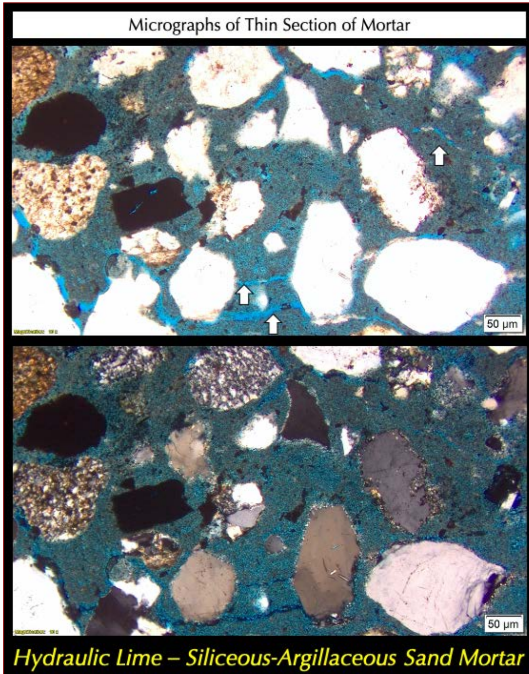
Figure 10: Micrographs of thin section of mortar showing: (a) non-air-entrained nature of mortar; (b) subangular to subrounded, mostly equidimensional siliceous-argillaceous sand particles that are nominal 2 mm in size, well-graded, well-distributed, consisting of major amount of variably strained quartz and subordinate amounts of quartzite, feldspar, quartz siltstone, and other siliceous particles; and a subordinate amount of shale, ferruginous and argillaceous siltstone particles, and (c) carbonated hydraulic lime paste. Top photo shows the plane polarized view to highlight sand particles, carbonation shrinkage microcracks (a few are marked with arrows) and voids, whereas bottom photo shows corresponding cross polarized light image to show the sand types and carbonated paste.
