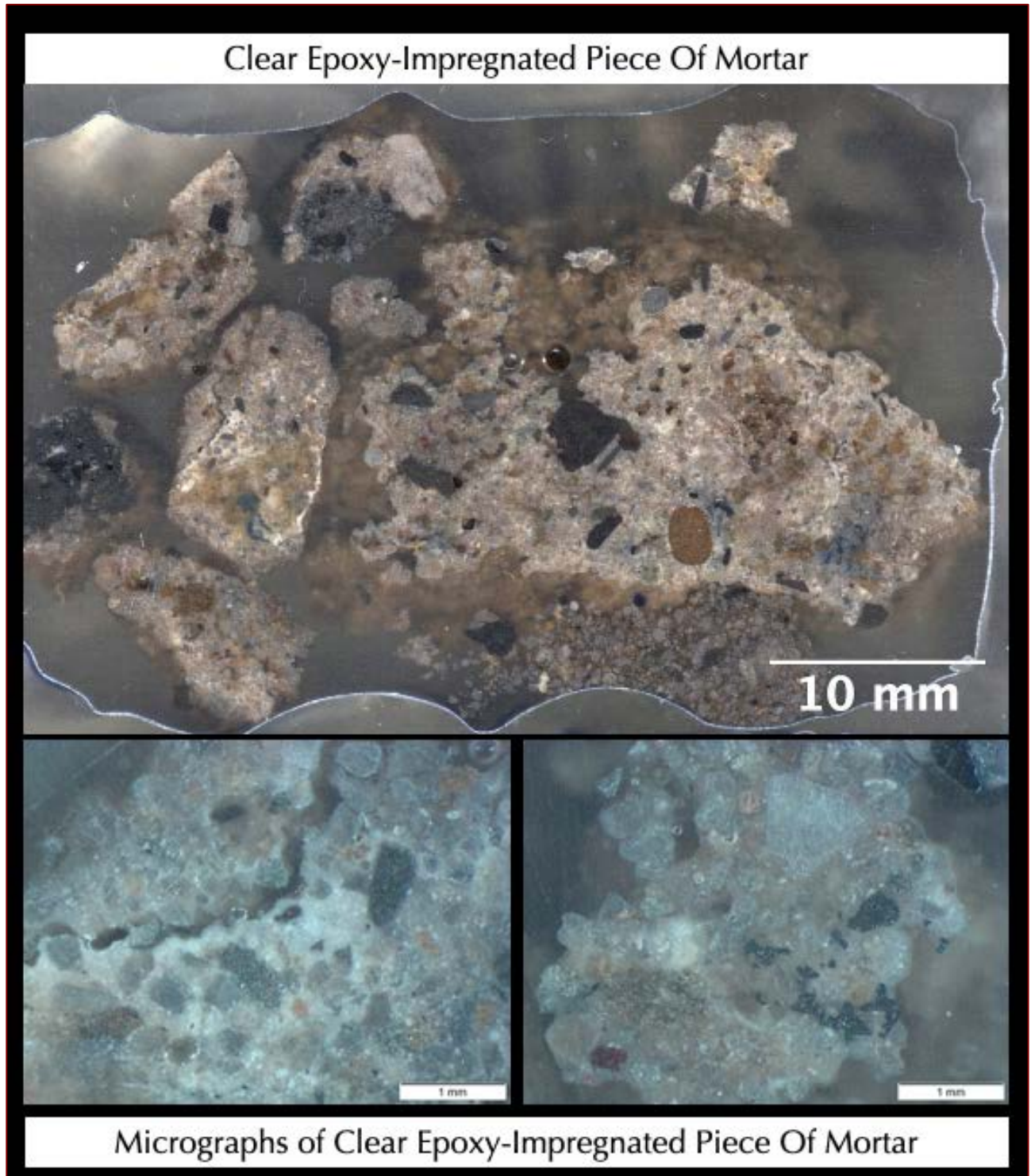
Figure 7: Clear epoxy-impregnated mortar showing size, shape, gradation, distribution, and color variations of sand particles, and interstitial paste fractions where color tone of the paste has somehow been masked with the clear epoxy. The bottom two photos are micrographs of clear epoxy-impregnated section where sand color variations and overall non-air-entrained nature of the mortar is seen.
