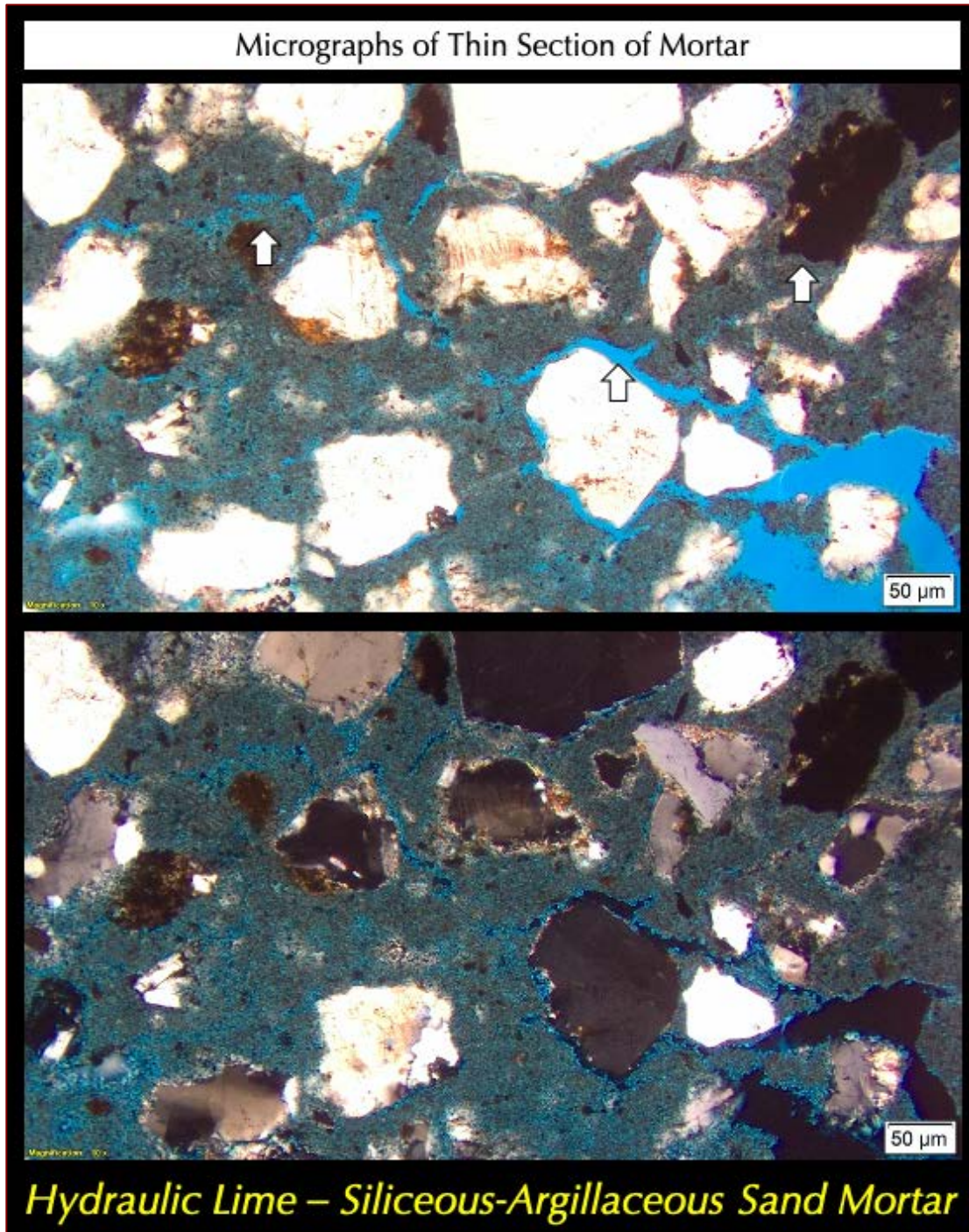
Figure 11: Micrographs of thin section of mortar showing: (a) non-air-entrained nature of mortar; (b) subangular to subrounded, mostly equidimensional siliceous-argillaceous sand particles that are nominal 2 mm in size, well-graded, well-distributed, consisting of major amount of variably strained quartz, and subordinate amounts of quartzite, feldspar, quartz siltstone, and other siliceous particles; and a subordinate amount of shale, ferruginous and argillaceous siltstone particles, and (c) carbonated hydraulic lime paste. Top photo shows the plane polarized view to highlight sand particles, carbonation shrinkage microcracks (a few are marked with arrows) and voids, whereas bottom photo shows corresponding cross polarized light image to show the sand types and carbonated paste.
