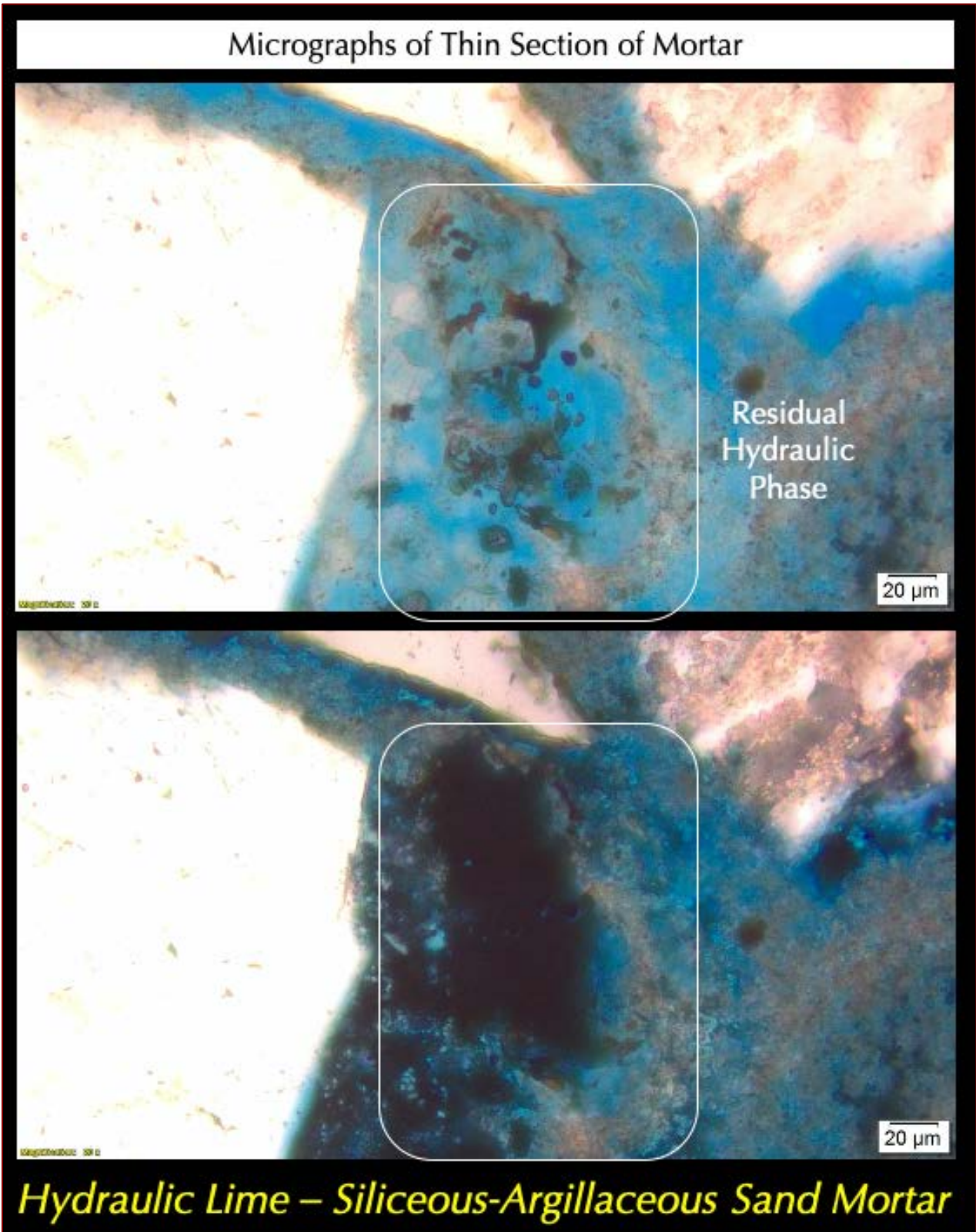
Figure 16: Micrographs of thin section of mortar showing a trace amount of residual hydraulic phases that are difficult to detect for their low abundance in the severely carbonated hydraulic lime paste. Notice the relic texture of the hydraulic phase where the dark brown interstitial ferrite-type phase is seen between the pseudomorphs of belite-type phases.
