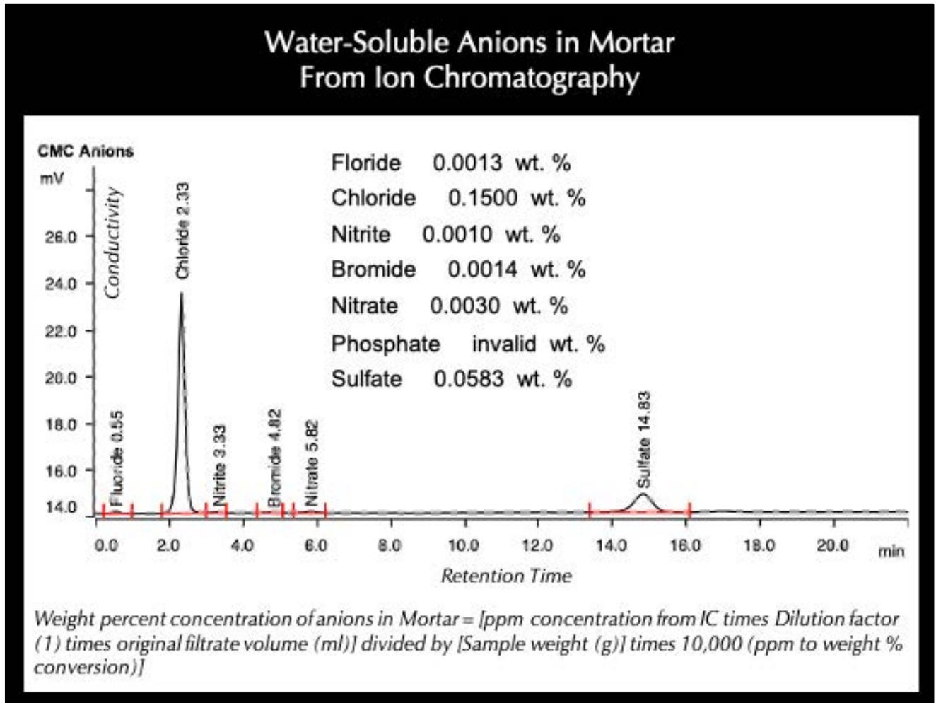
Figure 24: Ion chromatogram of water-soluble salt in mortar after digesting about a gram of pulverized mortar in deionized water for 30 minutes at a temperature below boiling, followed by continued digestion in water at the ambient laboratory condition for 24 hours. The filtrate was analyzed by ion chromatography. Results showed detectable chloride from the environment, minor sulfate from the Portland cement-free lime-based binder and sand, and negligible contents of other anions.
