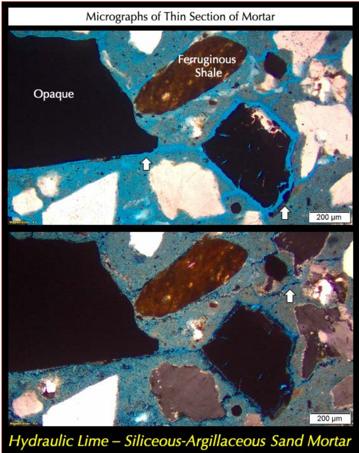
Figure 17: Micrographs of thin section of mortar showing: (a) non-air-entrained nature of mortar; (b) subangular to subrounded, mostly equidimensional siliceous-argillaceous sand particles that are nominal 2 mm in size, well-graded, well-distributed, consisting of major amount of variably strained quartz and subordinate amounts of quartzite, feldspar, quartz siltstone, and other siliceous particles; and a subordinate amount of shale, ferruginous and argillaceous siltstone particles, and (c) carbonated hydraulic lime paste. Top photo shows the plane polarized view to highlight sand particles, carbonation shrinkage microcracks (a few are marked with arrows) and voids, whereas bottom photo shows corresponding cross polarized light image to show the sand types and carbonated paste.
