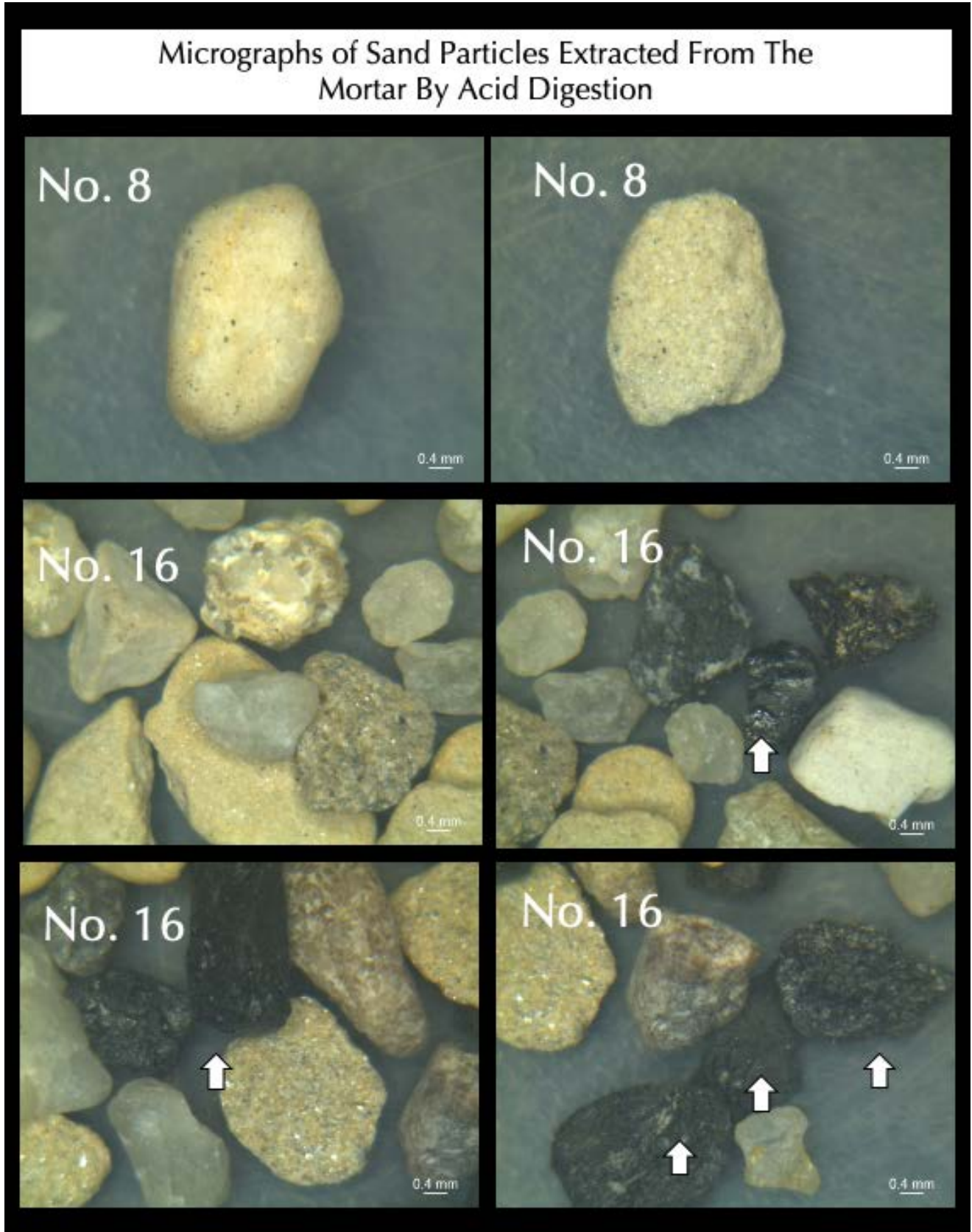
Figure 4: Micrographs of extracted sand particles from the mortar retained on various sieves. Arrows show some dark particles in sand.
