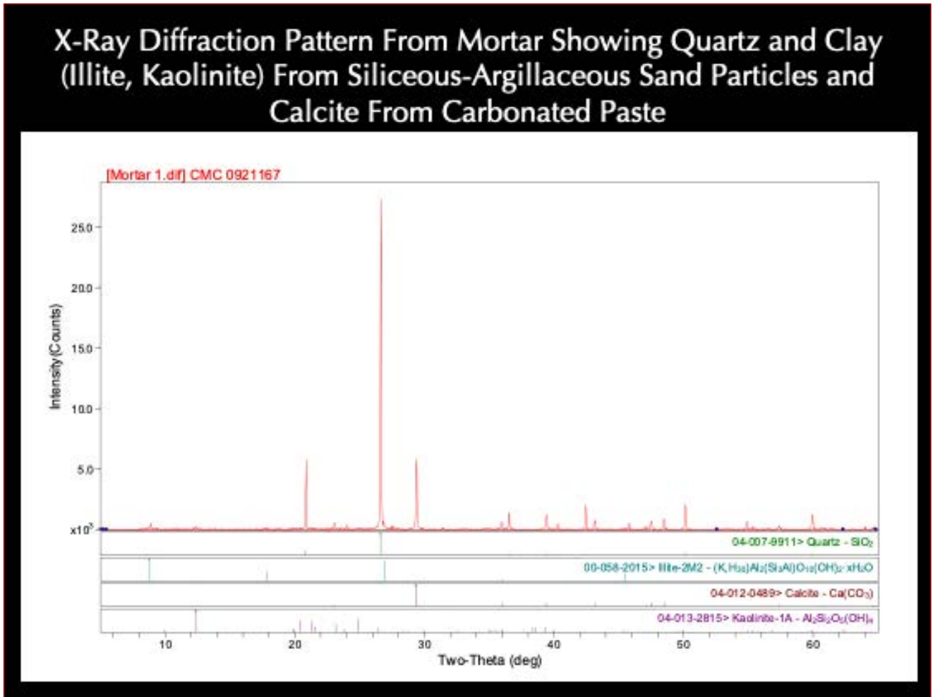
Figure 22: X-ray diffraction pattern of mortar showing the dominance of quartz from silica sand and subordinate calcite from carbonated cement paste. Illite and kaolinite-type clays detected are from the subordinate argillaceous component in the sand, which are potentially detrimental to the performance of mortar in the presence of moisture during service. Such clay components should be avoided in selection of mortar sand for the pointing mortar.
