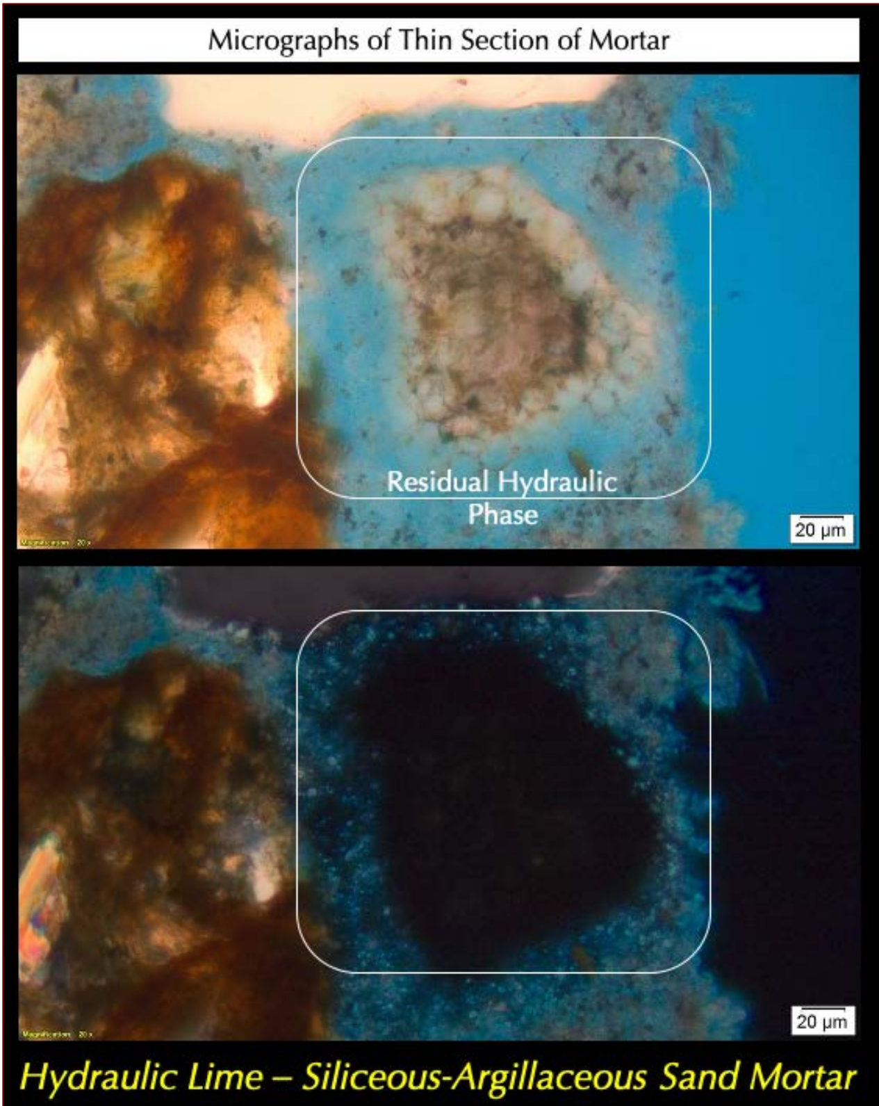
Figure 14: Micrographs of thin section of mortar showing a trace amount of residual hydraulic phases that are difficult to detect for their low abundance in the severely carbonated hydraulic lime paste. Notice the characteristic belite-type texture of the hydraulic phase as ‘bunch of grapes’, but overall isotropic nature due to dissolution in the bottom cross polarized light photo.
