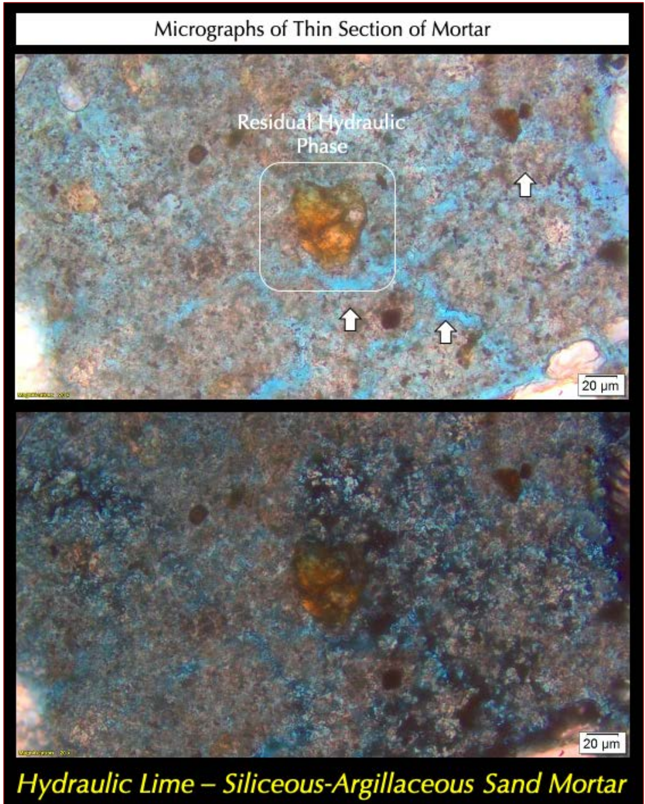
Figure 13: Micrographs of thin section of mortar showing a trace amount of residual hydraulic phases that are difficult to detect for their low abundance in the severely carbonated hydraulic lime paste.
