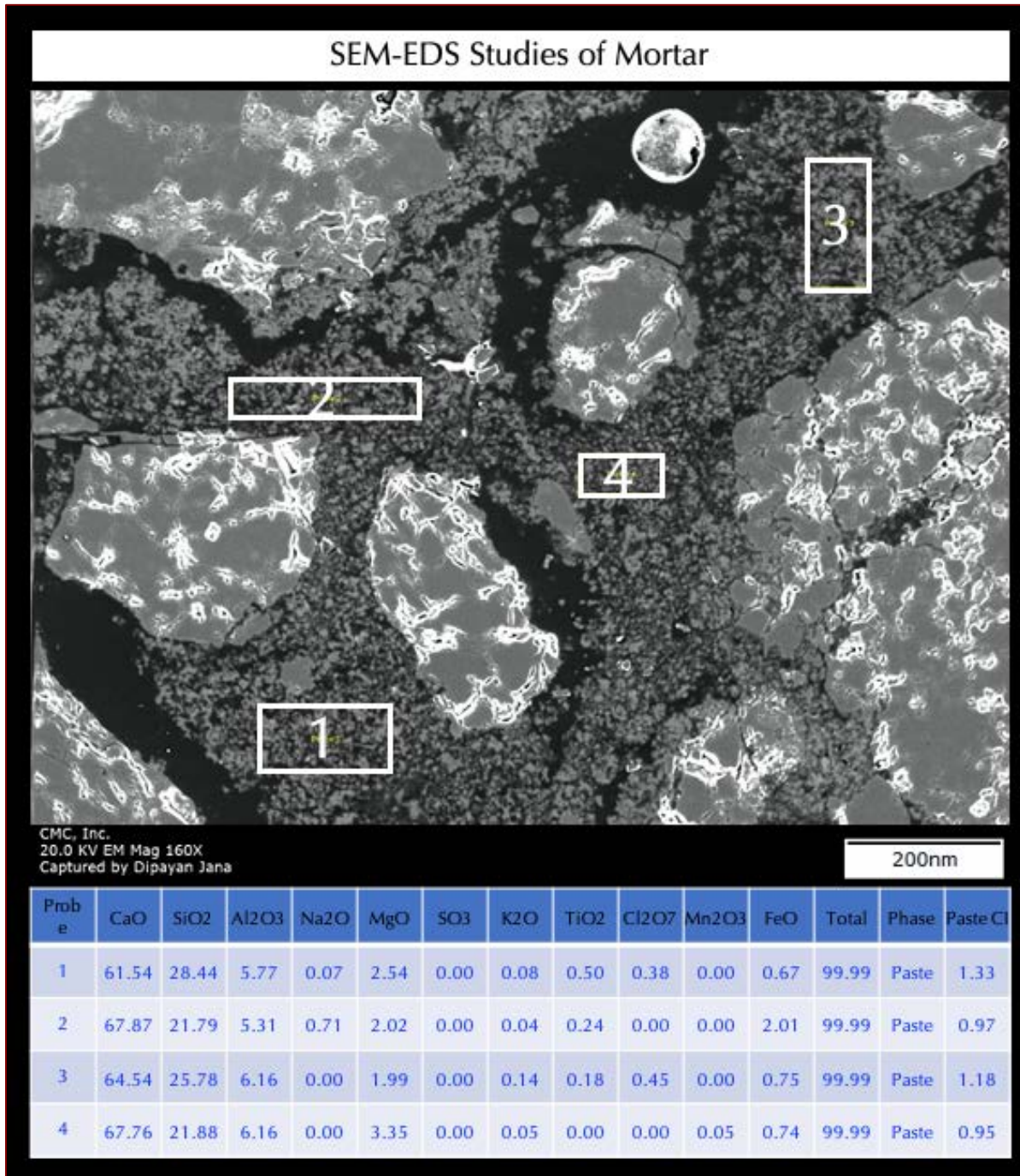
Figure 19: Secondary electron image (top), and X-ray microanalyses of boxed areas in Probes 1 through 4 detecting compositional variations of paste in the mortar. Paste compositions are presented (bottom) as oxide variations of all detected peaks normalized to 100% except carbon (from epoxy) and gold (from coating). Paste cementation indices, CI (after Eckel 1922) measure relative hydraulicity of paste e.g., non-hydraulic lime pastes have very low CI (< 0.50) compared to pastes of hydraulic phases and modern Portland cement pastes (CI is >1). Paste shows higher CI values (close to or >1) compared to non-hydraulic lime pastes (where CI is less than 0.5) indicating use of a hydraulic lime component. The cementation indices (CI) of paste are calculated after Eckel (1922) as CI = [(2.8 * SiO_2) + (1.1 * Al_2O_3) + (0.7 * Fe_2O_3)] / [(CaO) + (1.4 * MgO)] .
