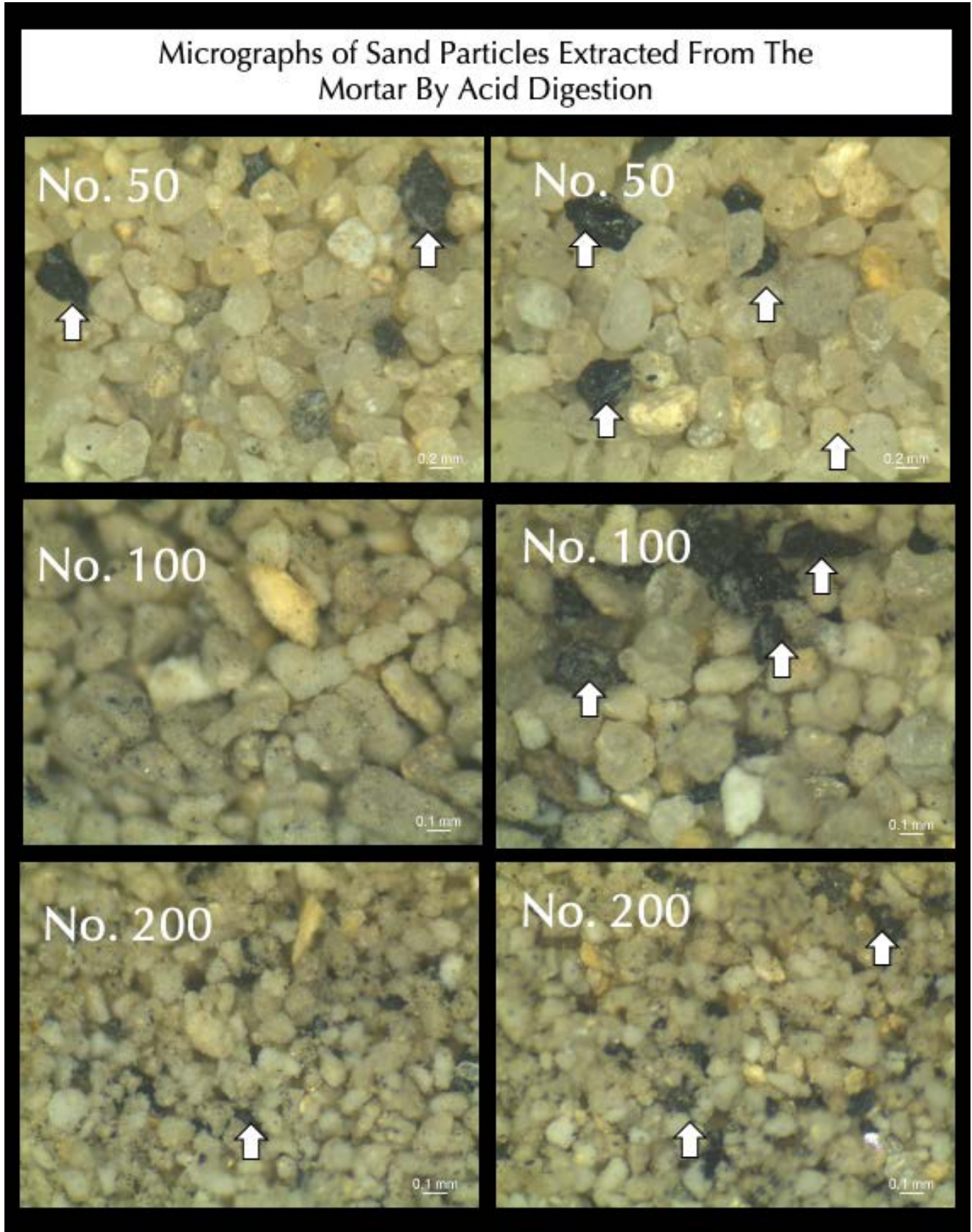
Figure 6: Micrographs of extracted sand particles from the mortar retained on various sieves. Arrows show some dark particles in sand.
