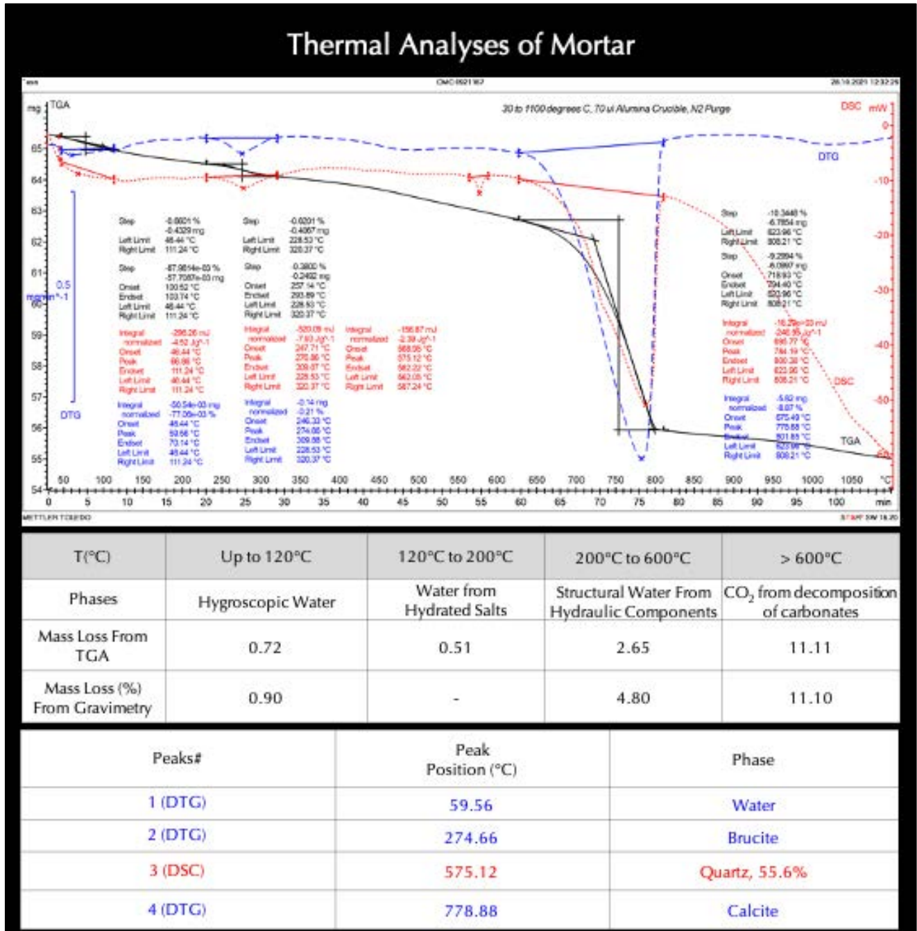
Figure 23: TGA (in bold black), DSC (in dotted red), and DTG (in dashed blue) curves of mortar showing losses in weight due to decompositions (loss of water and carbon dioxide) of various phases during controlled heating in a Mettler-Toledo’s simultaneous TGA/DSC 1 unit from 30°C to 1100°C in a ceramic crucible (alumina 70µl, no lid) at a heating rate of 10°C/min in a nitrogen purge at a rate of 75 mL/min. Dehydration and decarbonation reactions are marked as endothermic peaks in the DTG curve, whereas alpha to beta-form polymorphic transition of quartz is marked at the characteristic temperature of 575°C in the DSC curve. Similar results obtained from thermal analysis and gravimetry for mass losses from loss of free water (up to 120°C), structural water (200 to 600°C), and carbonation (600 to 950 °C), respectively. Quantitative estimate of quartz is determined from the DSC results. Notice the brucite peak at 274.66 °C is from the use of dolomitic lime binder in the mortar.
