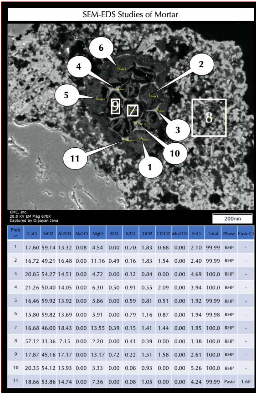
Figure 21: Secondary electron image (top), and X-ray microanalyses at the tips of callouts in Probes 1 through 11 detecting compositional variations of various phases within the residual hydraulic phase (RHP) in the hydraulic binder.
