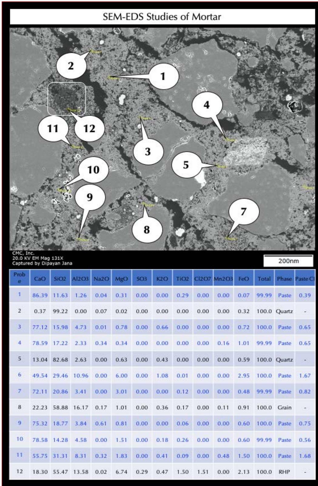
Figure 20: Secondary electron image (top), and X-ray microanalyses at the tips of callouts in Probes 1 through 12 detecting compositional variations of paste in the mortar. Within the boxed area is a residual hydraulic phase (RHP), which is analyzed in detail in the next Figure.
