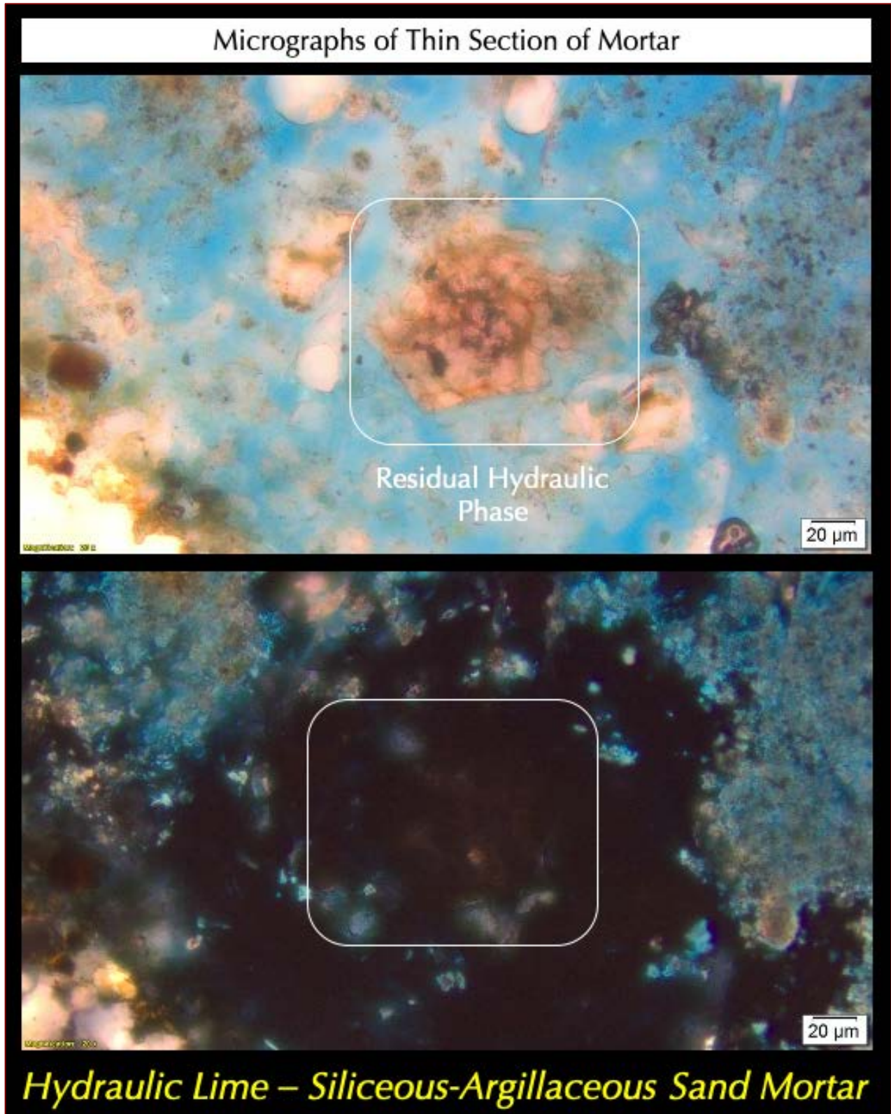
Figure 15: Micrographs of thin section of mortar showing a trace amount of residual hydraulic phases that are difficult to detect for their low abundance in the severely carbonated hydraulic lime paste. Notice the characteristic belite-type texture of the hydraulic phase as ‘bunch of grapes’ but overall isotropic nature due to dissolution in the bottom cross polarized light photo.
