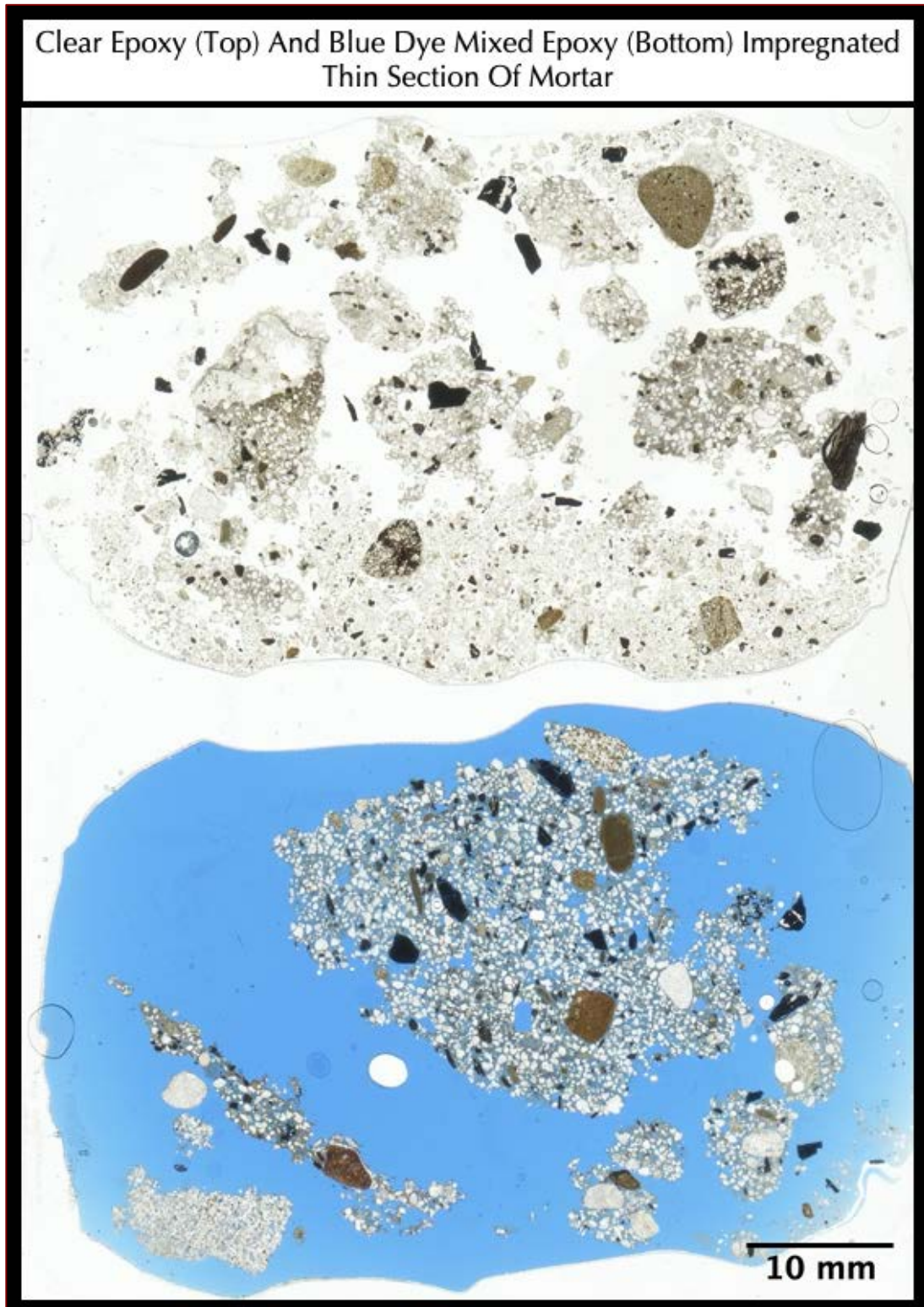
Figure 8: Blue dye-mixed epoxy-encapsulated thin section of mortar taken by using a flatbed film scanner, where thin section was scanned with a polarizing filter to recreate plane polarized light view of samples to show sand grain size, shape, angularity, and distribution, and pore and void spaces in mortar from blue epoxy (bottom).
