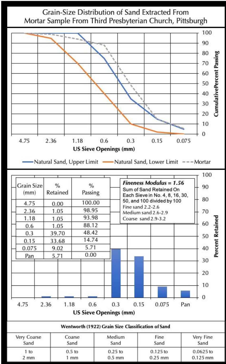
Figure 3: Grain-size distribution of sand extracted from the mortar.
