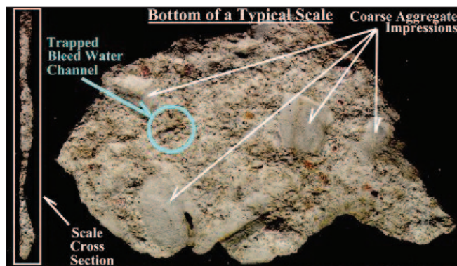
Figure 1. Features on the bottom of a scale.
