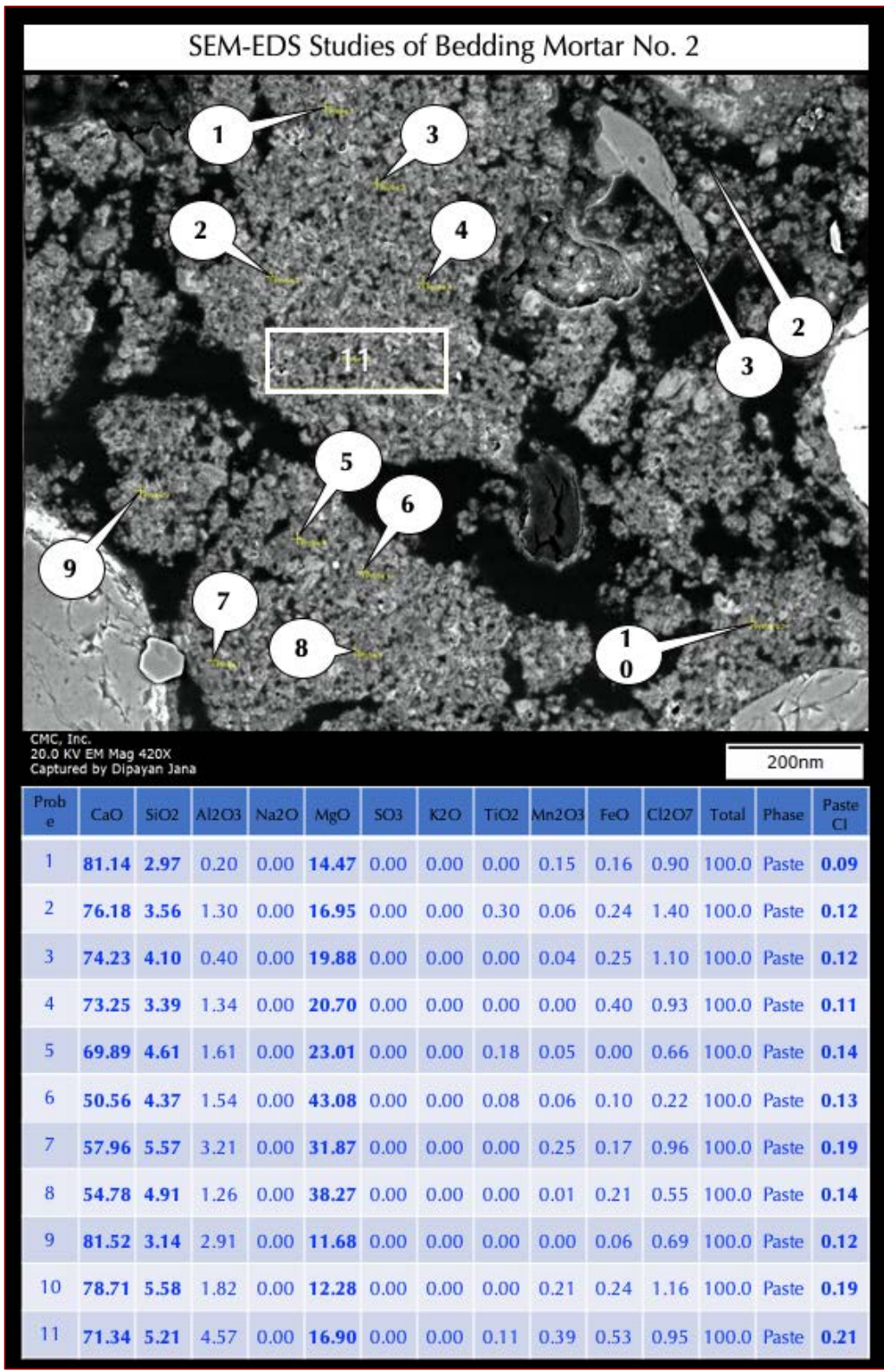
Figure 29: Secondary electron image (top), and X-ray microanalyses at the tips of callouts and in a boxed area in Probes 1 through 11 detecting compositional variations of paste in the bedding mortar No. 2.
