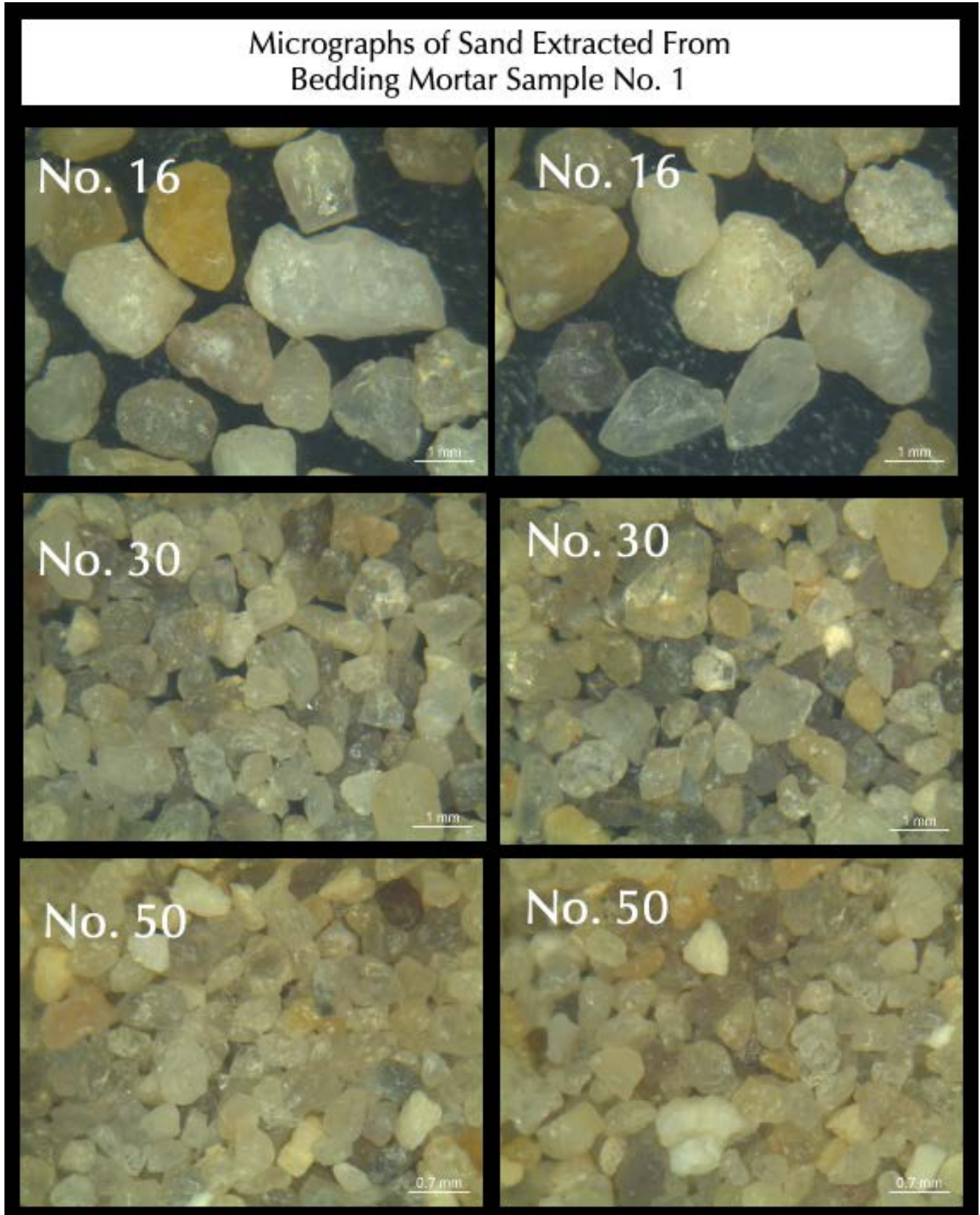
Figure 4: Micrographs of extracted sand from bedding mortar No. 1 retained on US Sieve Nos. 16, 30, and 50.
