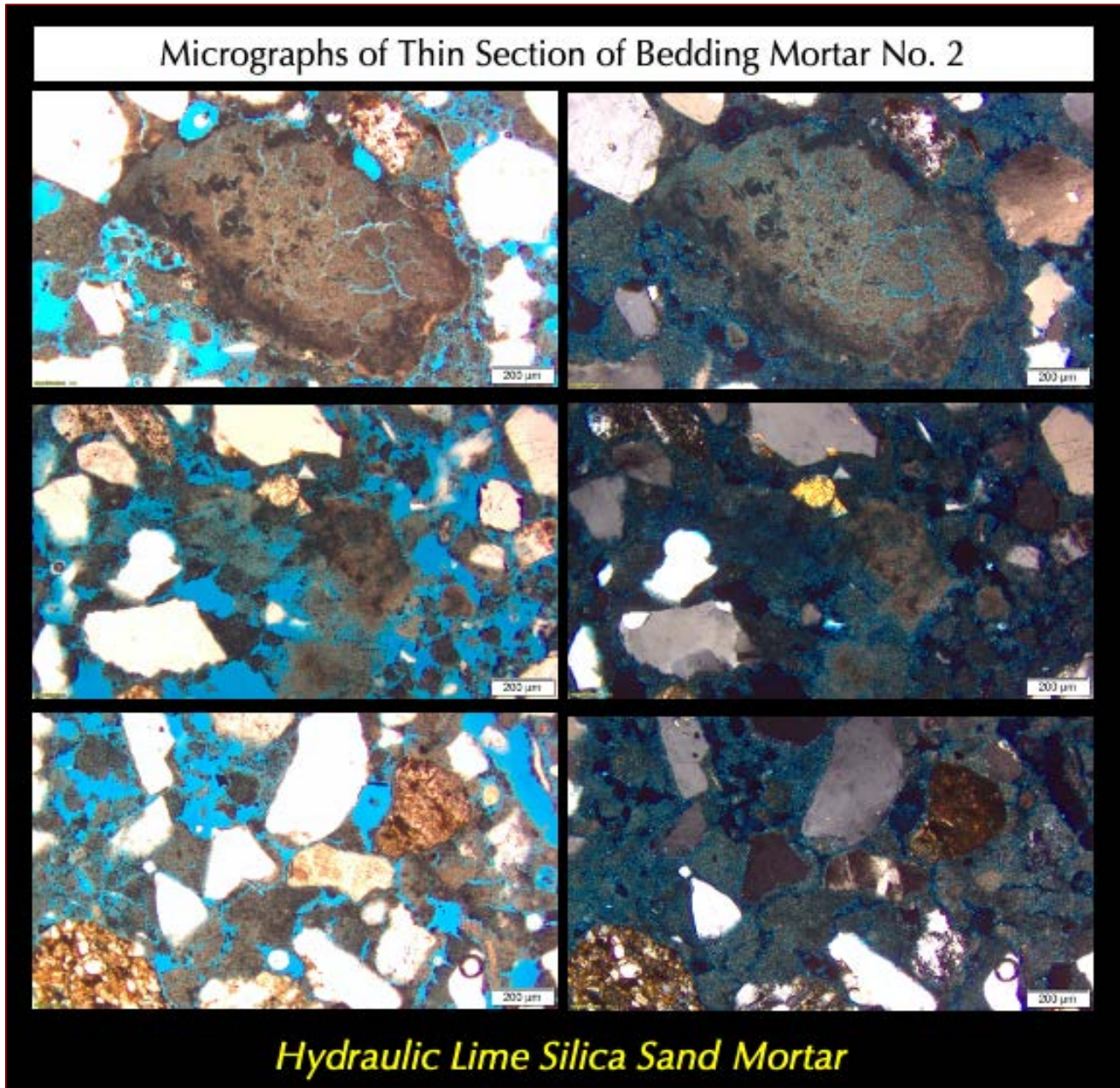
Figure 23: Micrographs of thin section of bedding mortar No. 2 showing: (a) a unmixed carbonated lime lump with internal microcracks in the top row, which are common in many historic lime mortars, (b) non-air-entrained nature of mortar; (c) subangular to subrounded, mostly equidimensional sand particles that are nominal 2 mm in size, well-graded, well-distributed, consisting of major amount of variably strained quartz and subordinate amounts of quartzite, feldspar, quartz siltstone, and other siliceous particles; and (d) a fine-grained, porous, severely carbonated paste, having short, discontinuous carbonation-shrinkage microcracks, all of which are common microstructural features of many historic lime mortars. Left column shows the plane polarized view to highlight sand particles and voids, whereas right column shows corresponding cross polarized light images to show siliceous composition of sand and carbonated paste.
