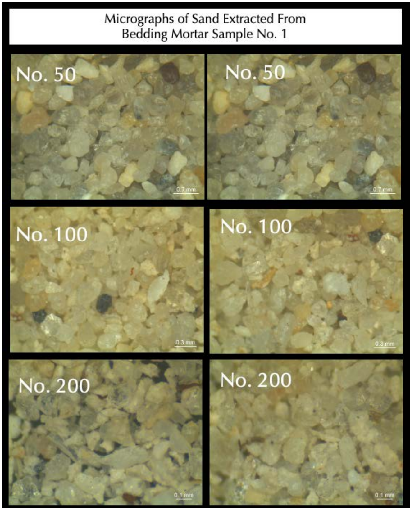
Figure 5: Micrographs of extracted sand from bedding mortar No. 1 retained on US Sieve Nos. 50, 100, and 200.
