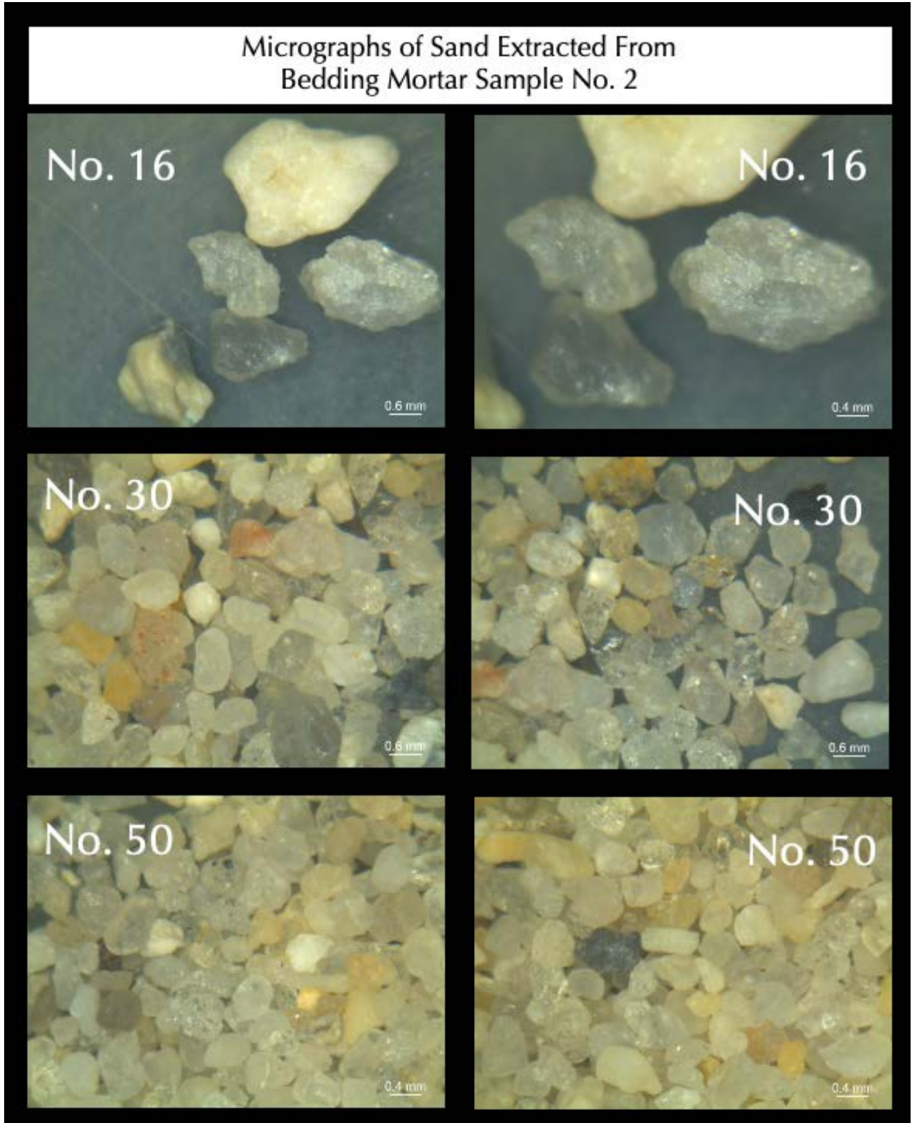
Figure 7: Micrographs of extracted sand from bedding mortar No. 2 retained on US Sieve Nos. 16, 30, and 50.
