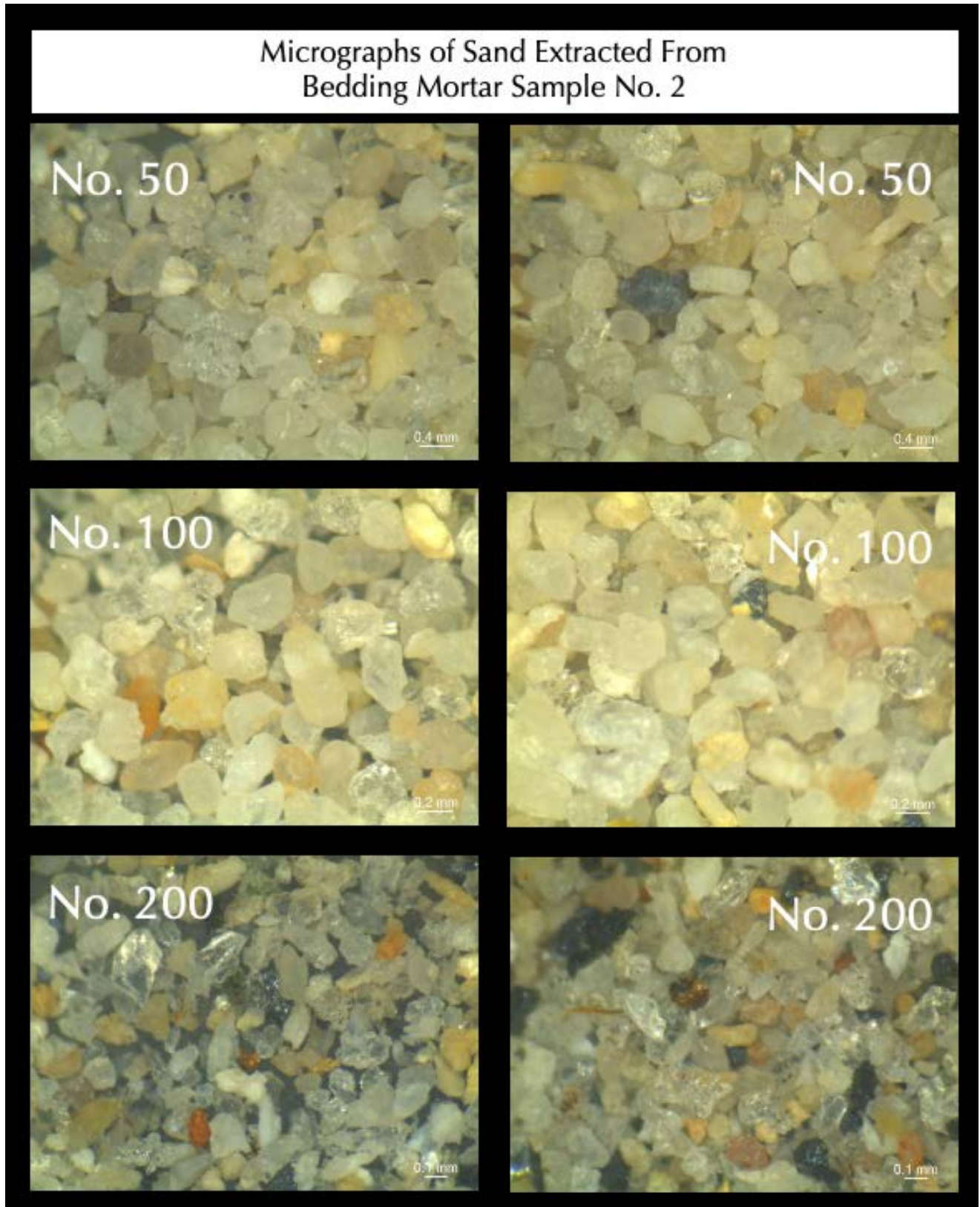
Figure 8: Micrographs of extracted sand from bedding mortar No. 2 retained on US Sieve Nos. 50, 100, and 200.
