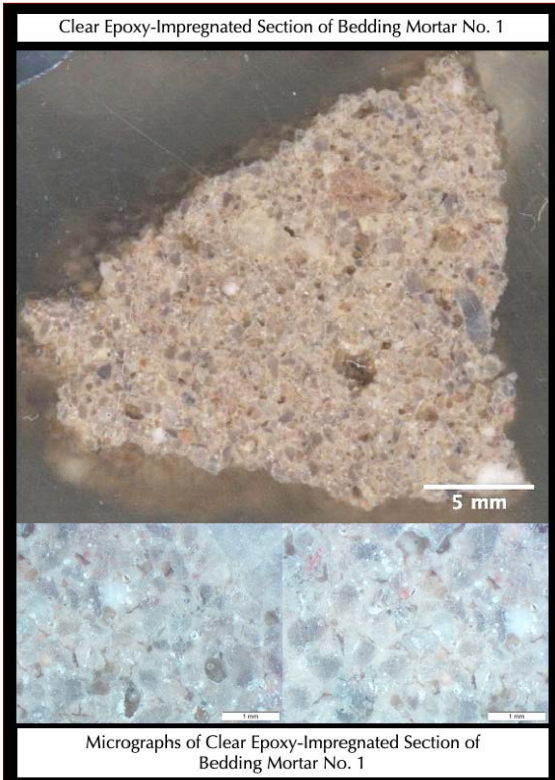
Figure 11: Clear epoxy encapsulated section of a bedding mortar piece from No. 1 in the top photo showing sand size, shape, angularity, color variations, gradation, and distribution across the mortar, and, the interstitial paste fraction. The bottom photo shows two micrographs from the top where sand particles and interstitial paste are seen. Notice lack of air entrainment in the mortar.
