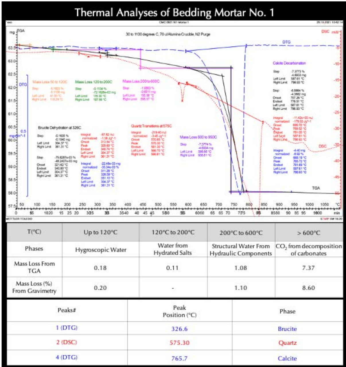
Figure 34: TGA (in bold black), DSC (in dotted red), and DTG (in dashed blue) curves of bedding mortar No. 1 showing losses in weight due to decompositions (loss of water and carbon dioxide) of various phases during controlled heating in a Mettler-Toledo’s simultaneous TGA/DSC 1 unit from 30°C to 1100°C in a ceramic crucible (alumina 70µl, no lid) at a heating rate of 10°C/min in a nitrogen purge at a rate of 75 mL/min. Dehydration and decarbonation reactions are marked as endothermic peaks in the DTG curve, whereas alpha to beta-form polymorphic transition of quartz is marked at the characteristic temperature of 575°C in the DSC curve. Similar results obtained from thermal analyses and gravimetry for mass losses from loss of free water (up to 120°C), structural water (200 to 600°C), and carbonation (600 to 950 °C), respectively. A shallow endothermic peak for brucite indicates magnesium composition of lime.
