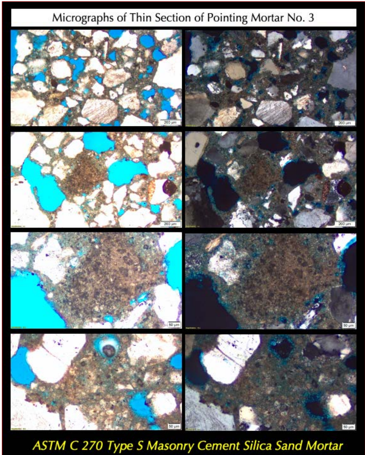
Figure 26: Micrographs of thin section of pointing mortar No. 3 showing: (a) a carbonated masonry cement paste having many residual Portland cement particles many of which are concentrated in unmixed neat cement paste lump in the 3 rd row, and minor amount of limestone fine particles; (b) air entrainment having many fine spherical entrained air-voids that are also characteristic of masonry cement mortars, as well as a few coarse irregular-shaped entrapped voids; and, (c) natural siliceous sand containing major amount of variably strained quartz and subordinate amounts of quartzite, feldspar, and other minor siliceous, argillaceous, and ferruginous particles.
