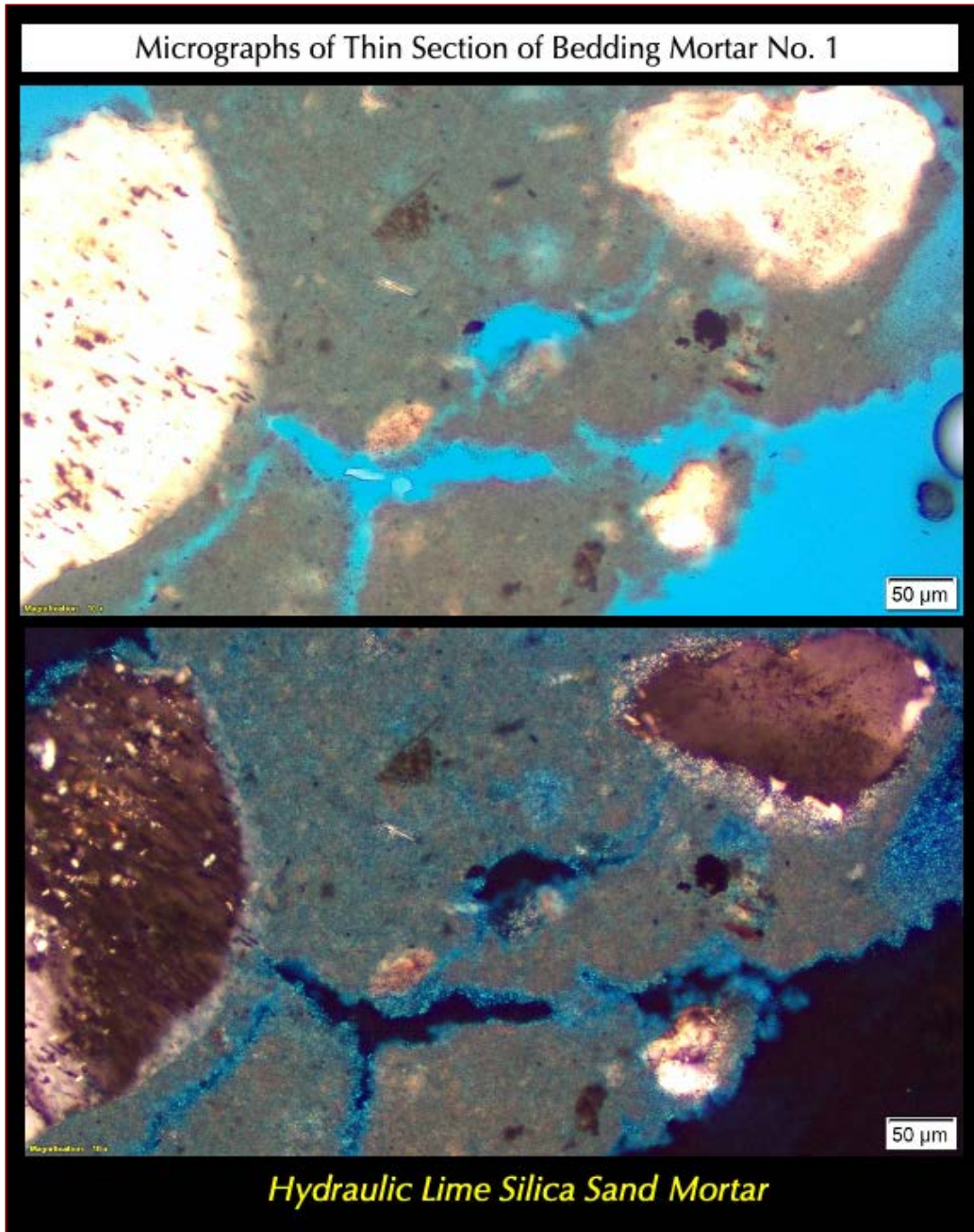
Figure 21: Micrographs of thin section of bedding mortar No. 1 showing: (a) non-air-entrained nature of mortar; (b) subangular to subrounded, mostly equidimensional sand particles that are nominal 2 mm in size, well-graded, well-distributed, consisting of major amount of variably strained quartz and subordinate amounts of quartzite, feldspar, quartz siltstone, and other siliceous particles; and, (c) a fine-grained, porous, severely carbonated paste, having short, discontinuous carbonation-shrinkage microcracks, all of which are common microstructural features of many historic lime mortars. Top photo shows the plane polarized view to highlight sand particles and voids, whereas bottom photo shows corresponding cross polarized light image to show siliceous composition of sand and carbonated paste.
