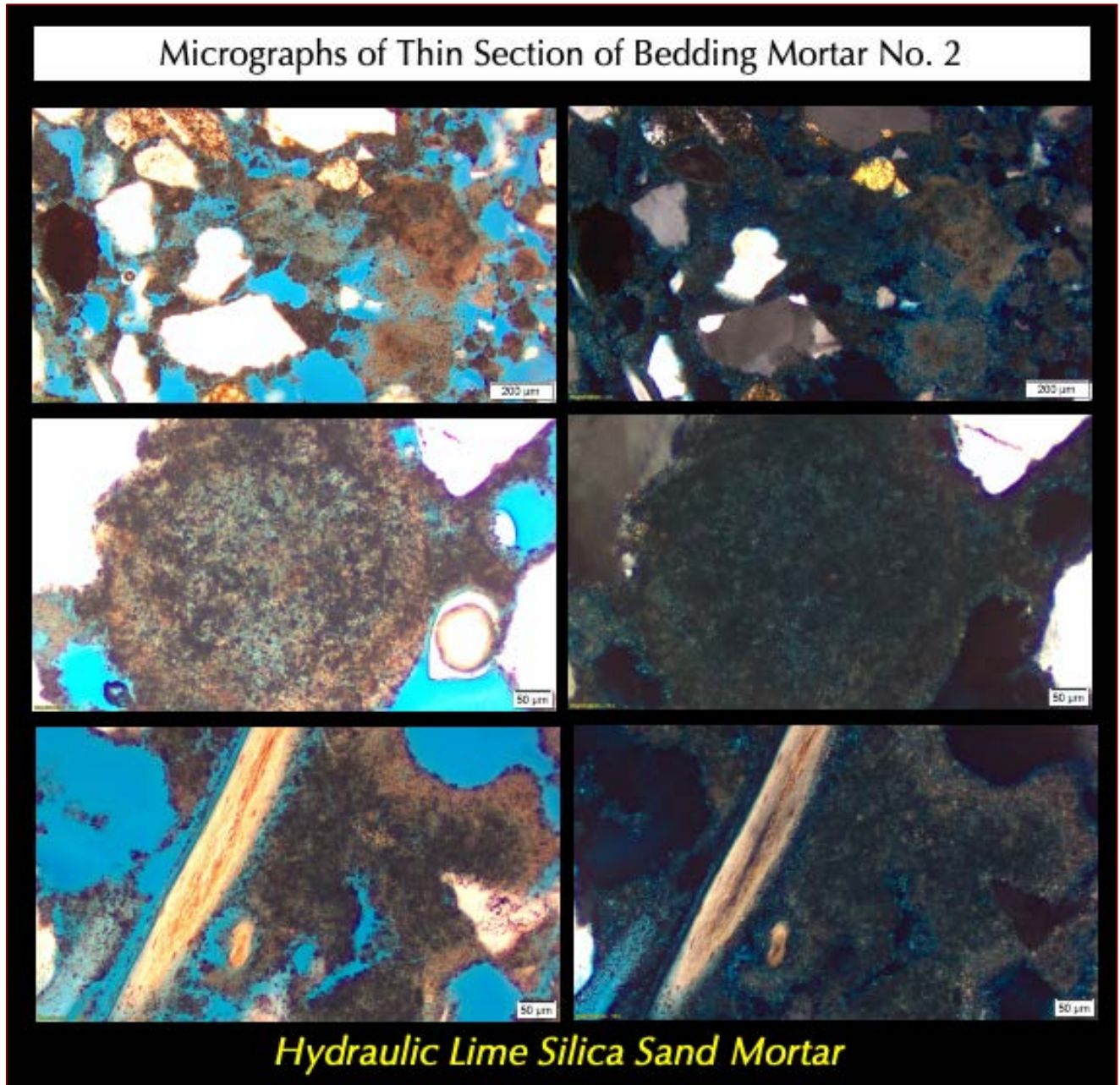
Figure 24: Micrographs of thin section of bedding mortar No. 2 showing: (a) an unmixed carbonated lime lump with internal microcracks in the middle row, which are common in many historic lime mortars, (b) non-air-entrained nature of mortar; (c) subangular to subrounded, mostly equidimensional sand particles that are nominal 2 mm in size, well-graded, well-distributed, consisting of major amount of variably strained quartz and subordinate amounts of quartzite, feldspar, quartz siltstone, and other siliceous particles; and (d) a fine-grained, porous, severely carbonated paste, having short, discontinuous carbonation-shrinkage microcracks, all of which are common microstructural features of many historic lime mortars. Left column shows the plane polarized view to highlight sand particles and voids, whereas right column shows corresponding cross polarized light images to show siliceous composition of sand and carbonated paste.
