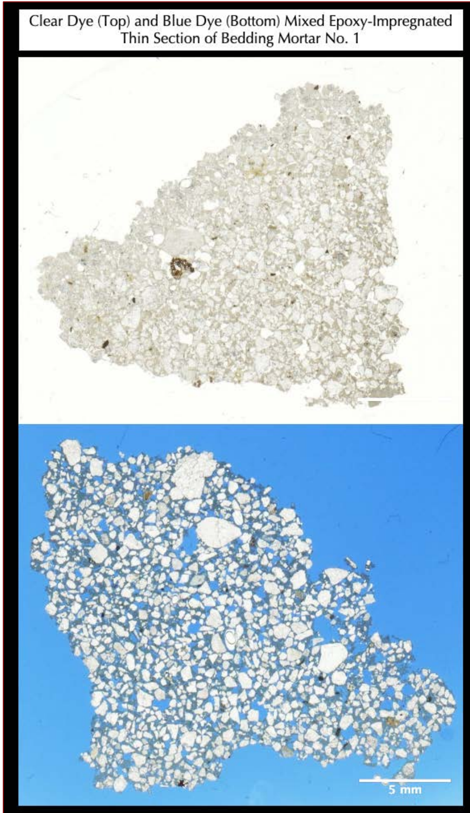
Figure 14: Clear epoxy (top) and blue dye-mixed epoxy (bottom) impregnated thin section of mortar fragment from the bedding mortar No. 1 taken by using a flatbed film scanner, where thin section was placed on a scanner with a polarizing filter to recreate plane polarized light view of sample to show the sand grain size, shape, angularity, and distribution, and, pore and void spaces in mortar from blue epoxy.
