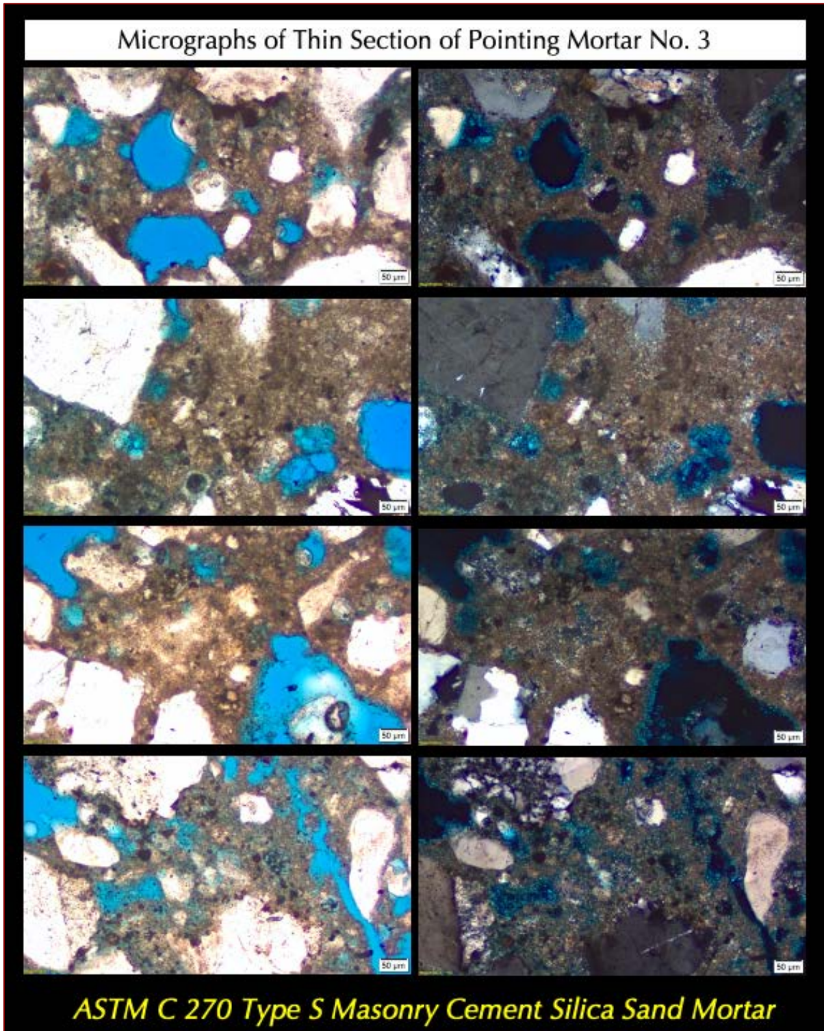
Figure 27: Micrographs of thin section of pointing mortar No. 3 showing: (a) a carbonated masonry cement paste having many residual Portland cement particles many of which are concentrated in unmixed neat cement paste lump in the 3 rd row, and minor amount of limestone fine particles; (b) air entrainment having many fine spherical entrained air voids that are also characteristic of masonry cement mortars, as well as a few coarse irregular-shaped entrapped voids; and (c) natural siliceous sand containing major amount of variably strained quartz and subordinate amounts of quartzite, feldspar, and other minor siliceous, argillaceous, and ferruginous particles.
