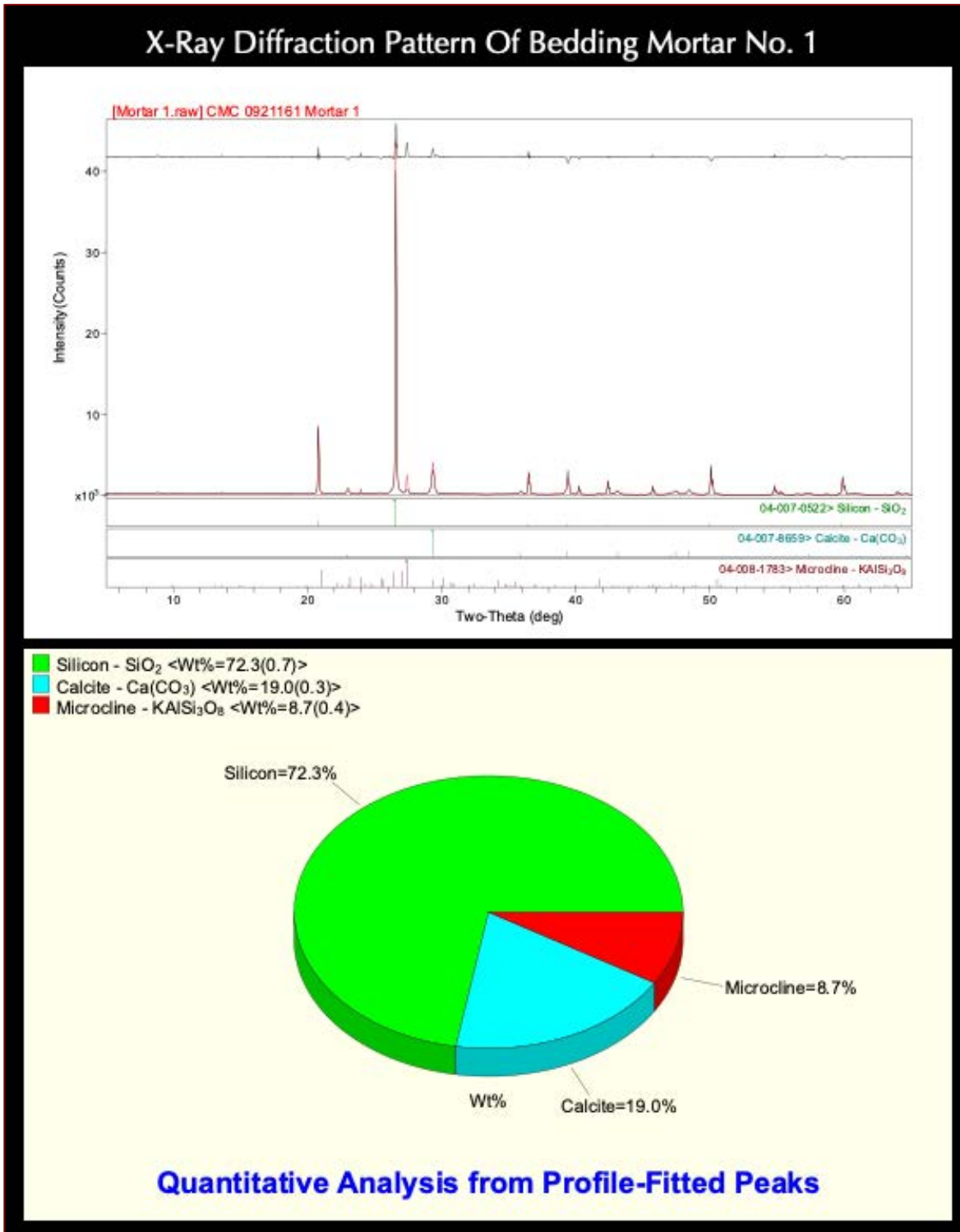
Figure 31: X-ray diffraction pattern of bedding mortar No. 1 showing the dominance of quartz and feldspar (microcline) from siliceous sand and subordinate calcite from carbonated cement paste. The bottom pie-graph shows relative proportions of quartz and calcite. Also detected is a trace amount of clay, which is not marked.
