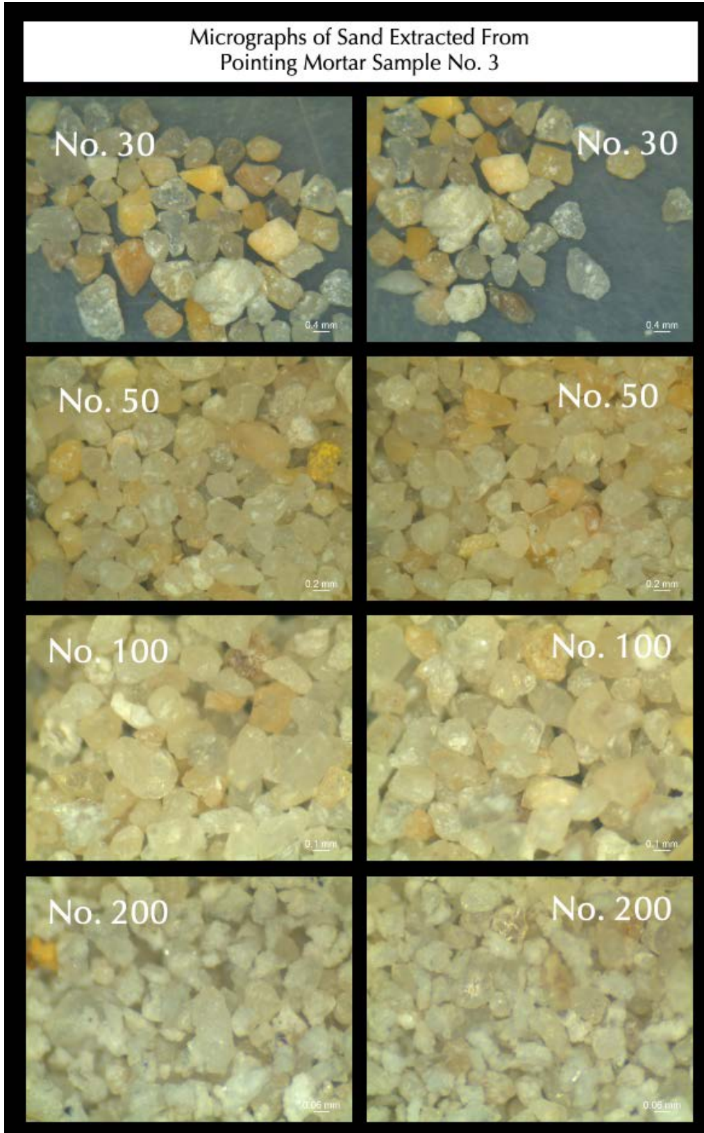
Figure 10: Micrographs of extracted sand from pointing mortar No. 3 retained on US Sieve Nos. 30, 50, 100, and 200.
