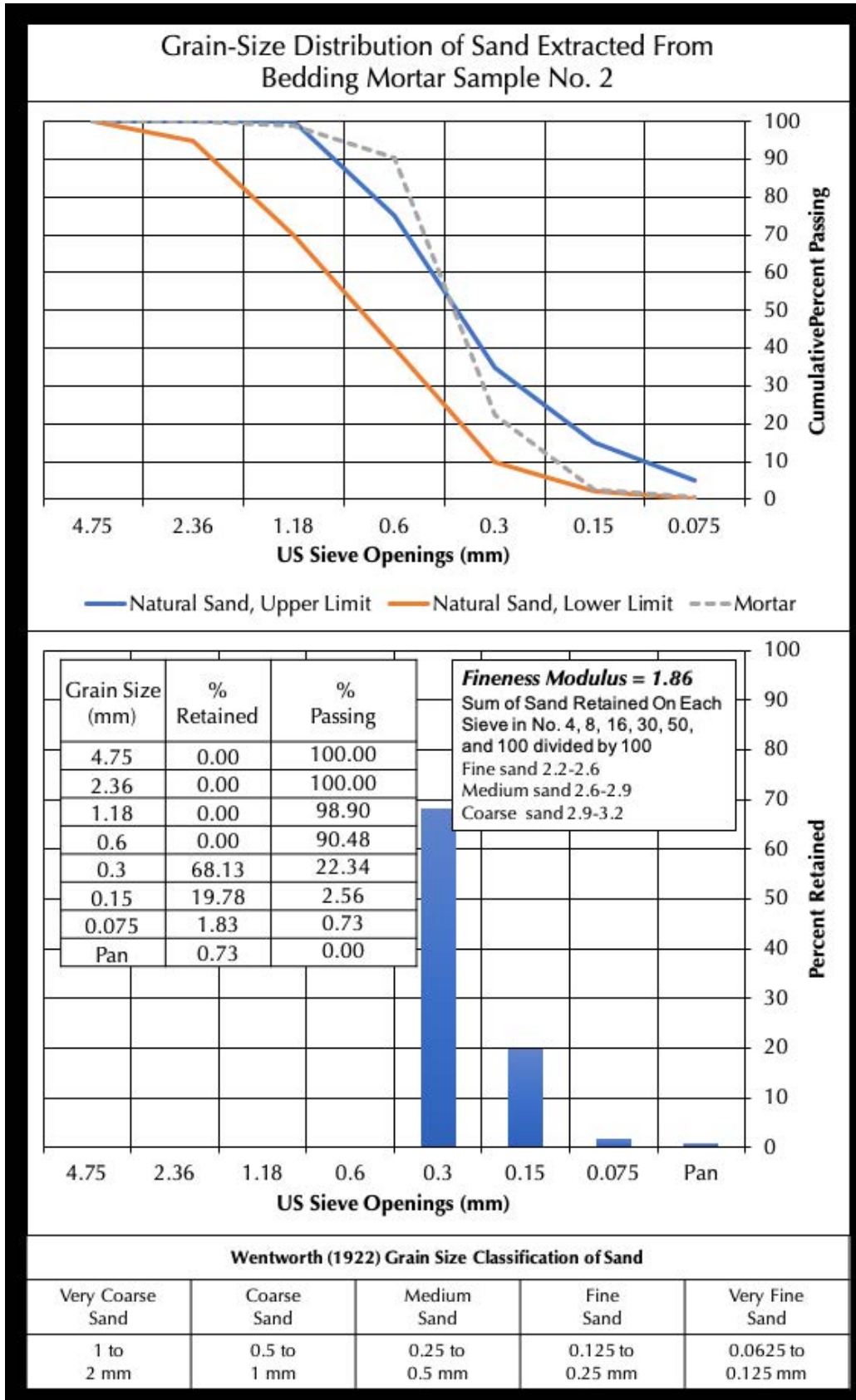
Figure 6: Grain-size distribution of sand extracted from the bedding mortar No. 2 after acid digestion.
