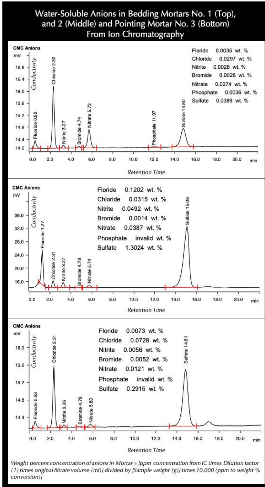
Figure 37: Ion chromatogram of water-soluble salts in all three mortars after digesting about a gram of pulverized mortar in deionized water for 30 minutes at a temperature below boiling, followed by continued digestion in water at the ambient laboratory condition for 24 hours. The filtrates were analyzed by ion chromatography.
