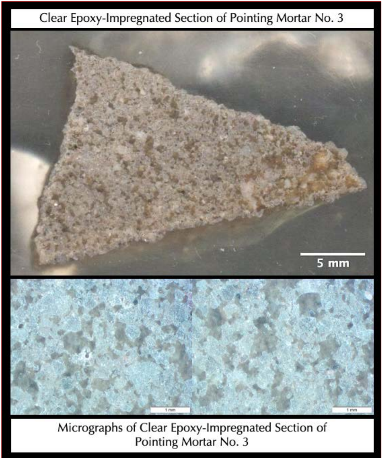
Figure 13: Clear epoxy encapsulated section of a pointing mortar piece from No. 3 in the top photo showing sand size, shape, angularity, color variations, gradation, and distribution across the mortar, and, the interstitial paste fraction. The bottom photo shows two micrographs from the top where sand particles and interstitial paste are seen. Notice abundant entrapped and interstitial voids that are filled with epoxy.
