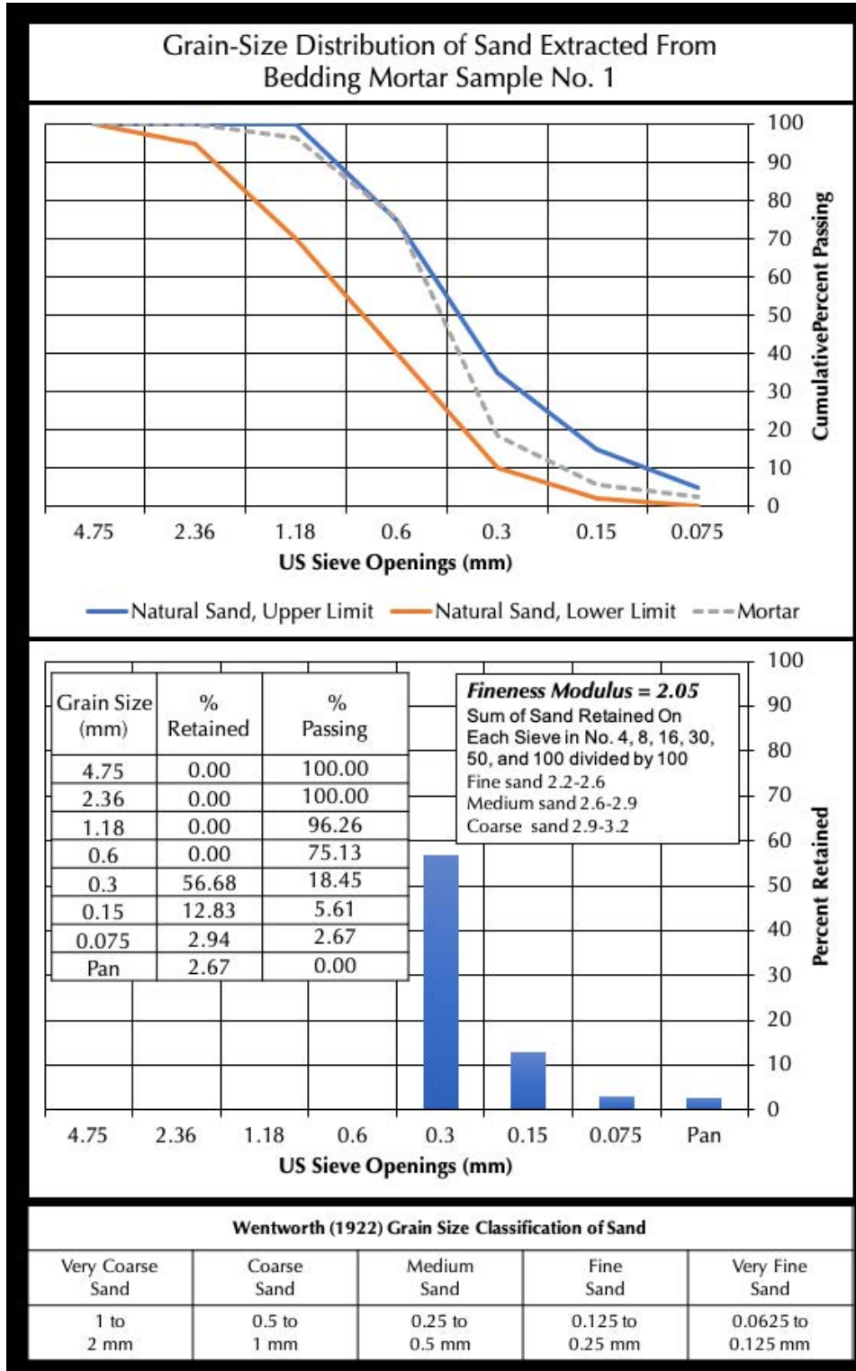
Figure 3: Grain-size distribution of sand extracted from the bedding mortar No. 1 after acid digestion.
