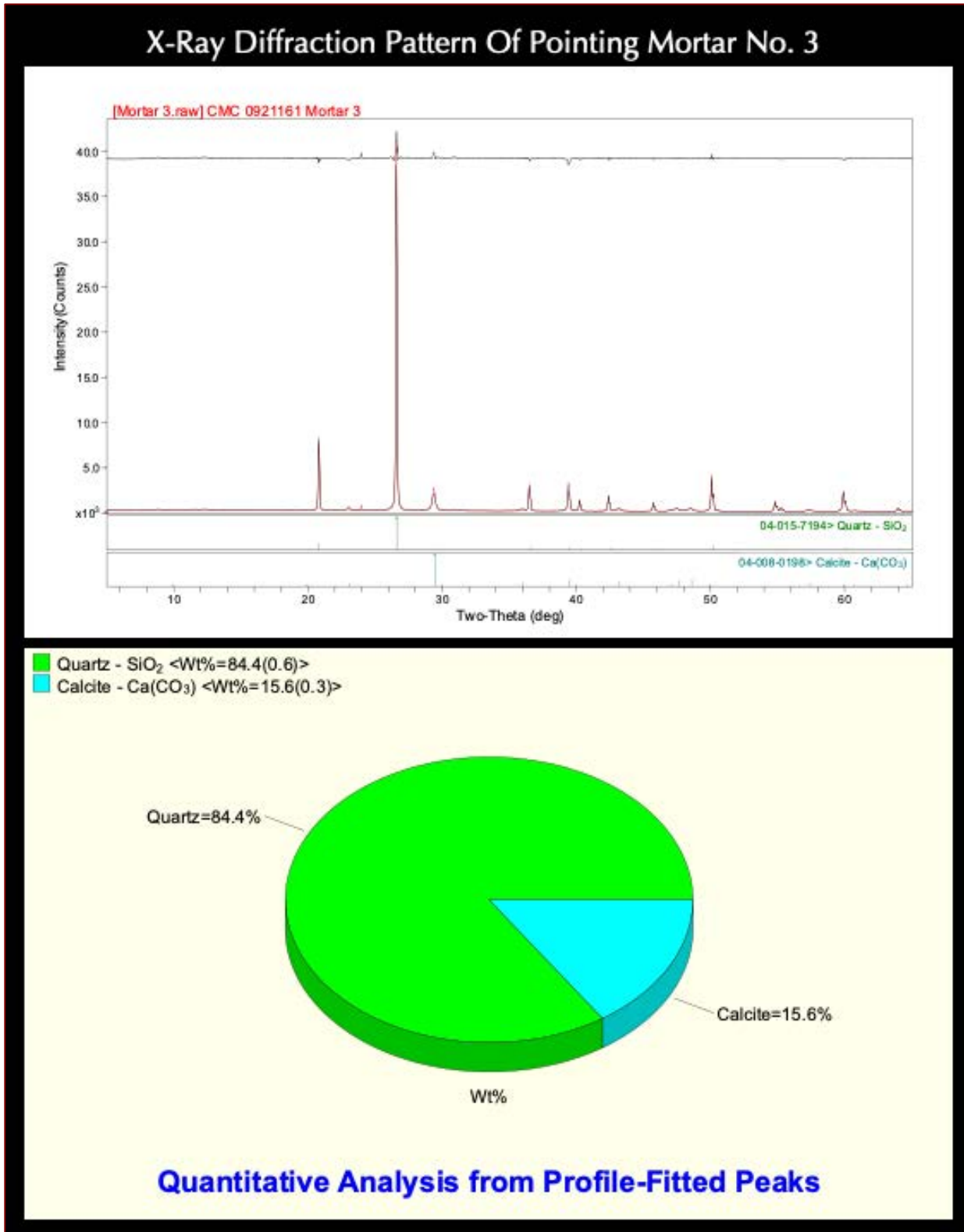
Figure 33: X-ray diffraction pattern of pointing mortar No. 3 showing the dominance of quartz from silica sand and subordinate calcite from carbonated cement paste. The bottom pie-graph shows relative proportions of quartz and calcite.
