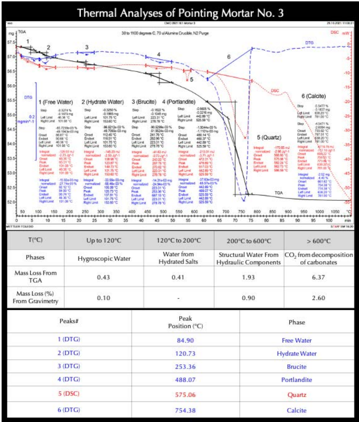
Figure 36: TGA (in bold black), DSC (in dotted red), and DTG (in dashed blue) curves of pointing mortar No. 3 showing losses in weight due to decompositions (loss of water and carbon dioxide) of various phases during controlled heating in a Mettler-Toledo's simultaneous TGA/DSC 1 unit from 30°C to 1100°C in a ceramic crucible (alumina 70µl, no lid) at a heating rate of 10°C/min in a nitrogen purge at a rate of 75 mL/min. Dehydration and decarbonation reactions are marked as endothermic peaks in the DTG curve, whereas alpha to beta-form polymorphic transition of quartz is marked at the characteristic temperature of 575°C in the DSC curve. Similar results obtained from thermal analyses and gravimetry for mass losses from loss of free water (up to 120°C), structural water (200 to 600°C), and carbonation (600 to 950 °C), respectively. A shallow endothermic peak for brucite indicates magnesium composition of lime component of binder. A peak at 488°C indicates non-carbonated hydrated lime component of the masonry cement binder.
