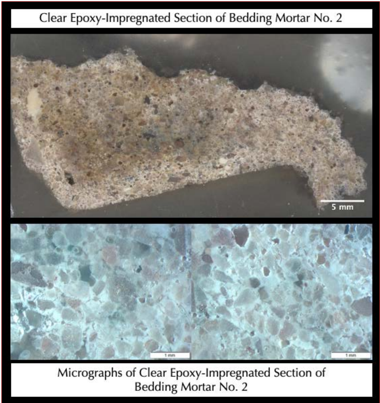
Figure 12: Clear epoxy encapsulated section of a bedding mortar piece from No. 2 in the top photo showing sand size, shape, angularity, color variations, gradation, and distribution across the mortar and the interstitial paste fraction. The bottom photo shows two micrographs from the top where sand particles and interstitial paste are seen. Notice lack of air entrainment in the mortar.
