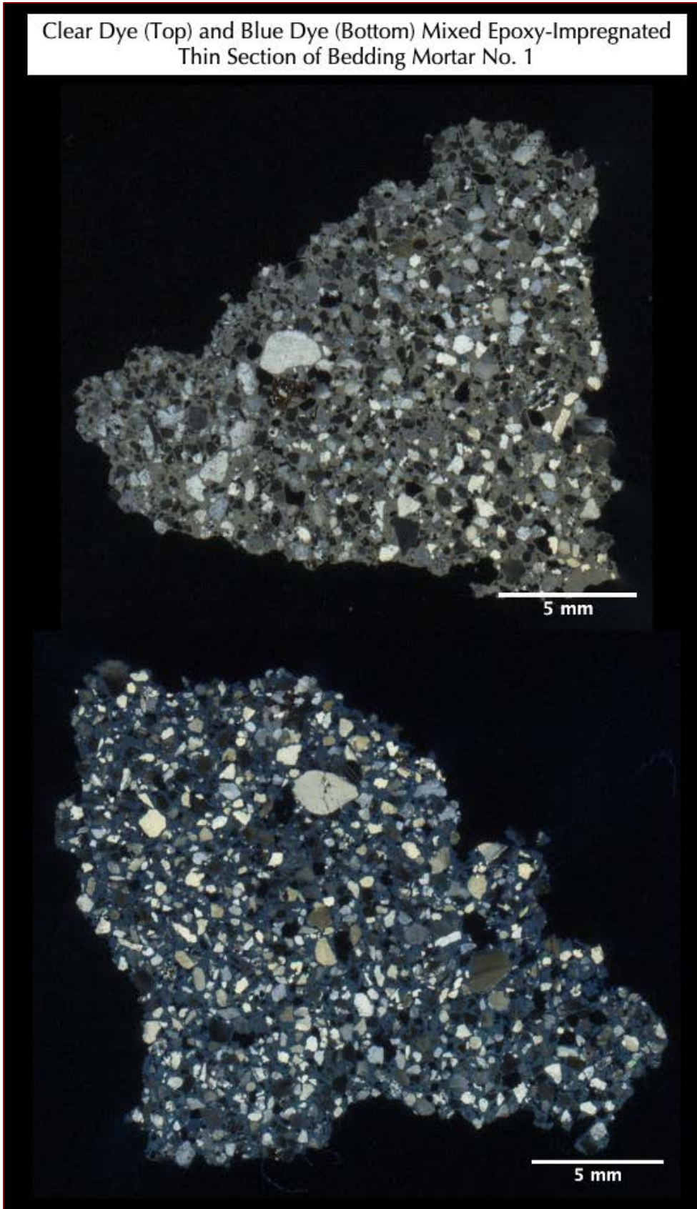
Figure 15: Clear epoxy (top) and blue dye-mixed epoxy (bottom) impregnated thin section of mortar fragment from the bedding mortar No. 1 taken by using a flatbed film scanner, where thin section was placed on a scanner with two perpendicular polarizing filters to recreate cross polarized light view of sample to show the siliceous composition of sand and variably carbonated paste.
