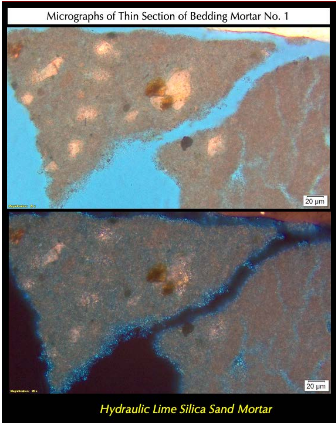
Figure 22: Micrographs of thin section of bedding mortar No. 1 showing fine-grained, porous, severely carbonated paste, having short, discontinuous carbonation-shrinkage microcracks, all of which are common microstructural features of many historic lime mortars. Top photo shows the plane polarized view to highlight sand particles and voids, whereas bottom photo shows corresponding cross polarized light image to show siliceous composition of sand and carbonated paste.
