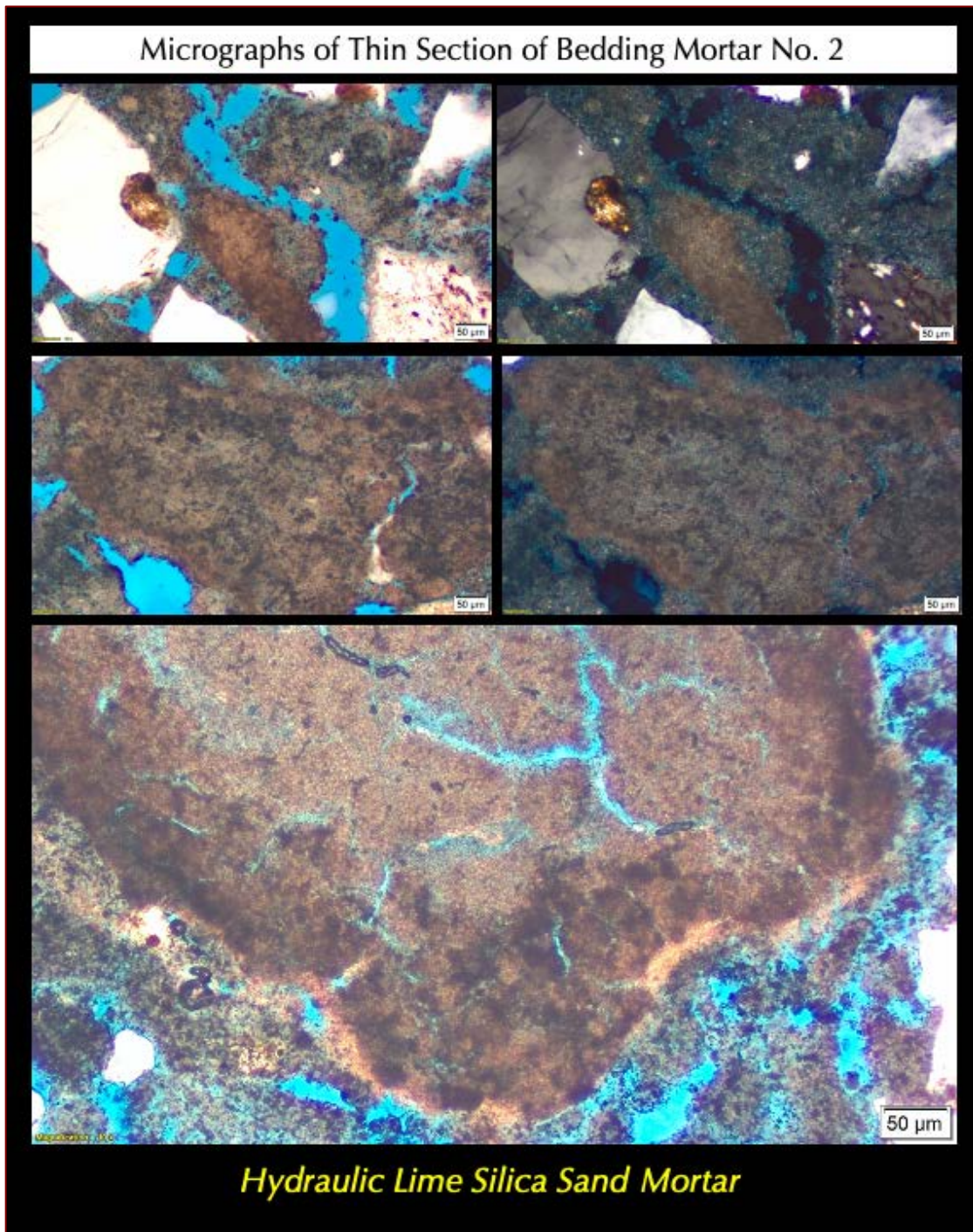
Figure 25: Micrographs of thin section of bedding mortar No. 2 showing: (a) an unmixed carbonated lime lump with internal microcracks in the middle and bottom rows, which are common in many historic lime mortars, (b) non-air-entrained nature of mortar; (c) subangular to subrounded, mostly equidimensional sand particles that are nominal 2 mm in size, well-graded, well-distributed, consisting of major amount of variably strained quartz and subordinate amounts of quartzite, feldspar, quartz siltstone, and other siliceous particles; and, (d) a fine-grained, porous, severely carbonated paste, having short, discontinuous carbonation-shrinkage microcracks, all of which are common microstructural features of many historic lime mortars. Left column shows the plane polarized view to highlight sand particles and voids, whereas right column shows corresponding cross polarized light images to show siliceous composition of sand and carbonated paste.
