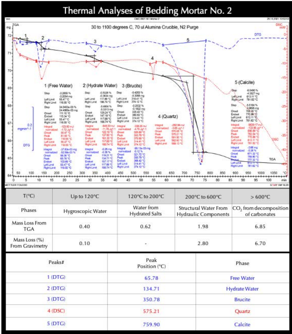
Figure 35: TGA (in bold black), DSC (in dotted red), and DTG (in dashed blue) curves of bedding mortar No. 2 showing losses in weight due to decompositions (loss of water and carbon dioxide) of various phases during controlled heating in a Mettler-Toledo’s simultaneous TGA/DSC 1 unit from 30°C to 1100°C in a ceramic crucible (alumina 70µl, no lid) at a heating rate of 10°C/min in a nitrogen purge at a rate of 75 mL/min. Dehydration and decarbonation reactions are marked as endothermic peaks in the DTG curve, whereas alpha to beta-form polymorphic transition of quartz is marked at the characteristic temperature of 575°C in the DSC curve. Similar results obtained from thermal analyses and gravimetry for mass losses from loss of free water (up to 120°C), structural water (200 to 600°C), and carbonation (600 to 950 °C), respectively. A strong endothermic peak for brucite (more distinct than No. 1) indicates dolomitic lime mortar, which is also consistent with noticeably higher magnesia contents of paste in No. 2 than in No. 1 bedding mortar. A strong endothermic peak at 134.7°C is from dehydroxylation of gypsum, which is also detected in the XRD analysis of this mortar.
