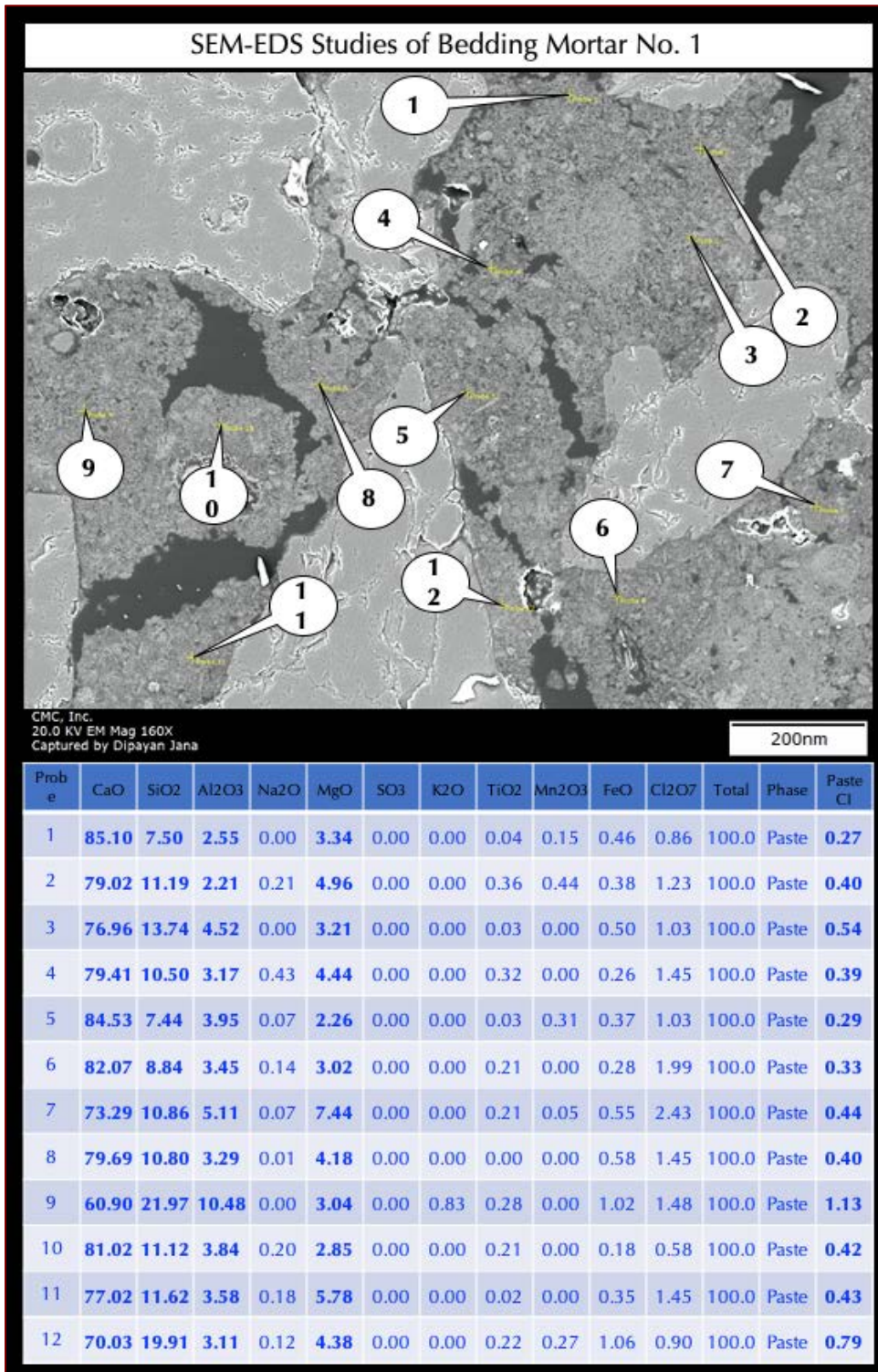
Figure 28: Secondary electron image (top), and X-ray microanalyses at the tips of callouts in Probes 1 through 12 detecting compositional variations of paste in the bedding mortar No. 1.
