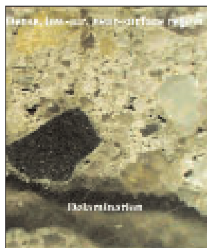
Figure 1, left: The cross section on the left shows a surface region from the warehouse floor where a dense low-air mortar devoid of coarse aggregate particles is underlain by a delamination plane. Air-entrained concrete in the rest of the core is shown on the right. Figure 2, below: These figures show profiles of air and paste contents of the core shown in Figure 1—the warehouse floor. The decreased air content (left) and increased paste content (right) in the top inch are due to finishing manipulations that washed air out of the surface region and forced coarse aggregate particles deeply into the concrete.
